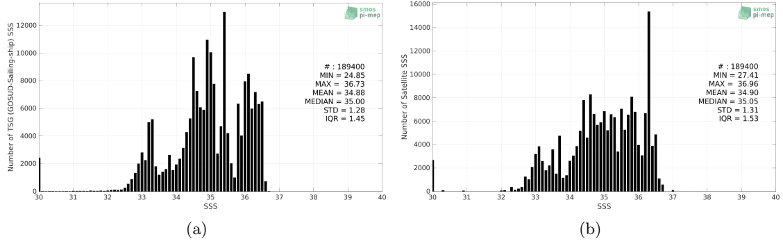
Figure 2: Histograms of SSS from TSG (GOSUD-Sailing-ship) (a) and SMOS SSS L3 v8 - 9 Days (CATDS-CECOS-LOCEAN) (b) considering all match-up pairs per bins of 0.1 over the Tropical Pacific Ocean Pi-MEP region and for the full satellite product period.
