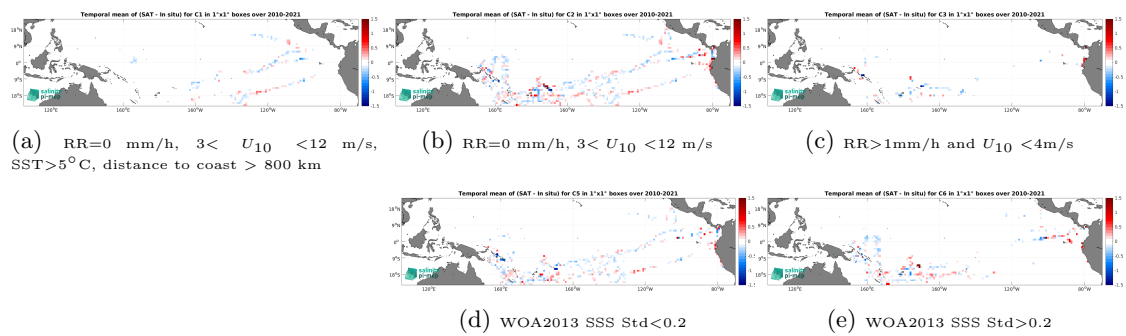
Figure 12: Temporal mean gridded over spatial boxes of size 1^\circ \times 1^\circ of \Delta SSS (SMOS SSS L3 v8 - 9 Days (CATDS-CEC-LOCEAN) - TSG (GOSUD-Research-vessel)) for 5 different subdatasets corresponding to:RR=0 mm/h, 3 < U_{10} < 12 m/s, SST > 5^\circ\text{C} , distance to coast > 800 km (a), RR=0 mm/h, 3 < U_{10} < 12 m/s (b), RR > 1 mm/h and U_{10} < 4 m/s (c), WOA2013 SSS Std < 0.2 (d), WOA2013 SSS Std > 0.2 (e).
