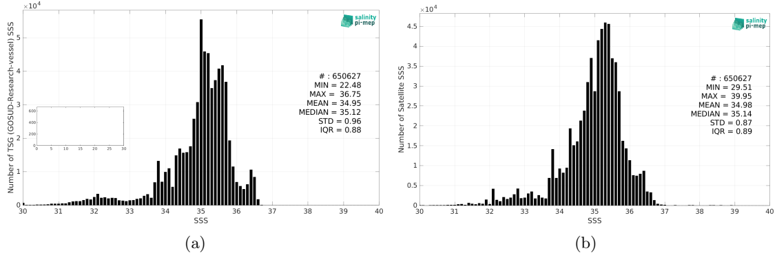
Figure 2: Histograms of SSS from TSG (GOSUD-Research-vessel) (a) and SMOS SSS L3 v8 - 9 Days (CATDS-CEC-LOCEAN) (b) considering all match-up pairs per bins of 0.1 over the Tropical Pacific Ocean Pi-MEP region and for the full satellite product period.
