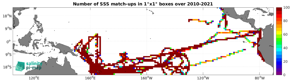
Figure 4: Number of SSS match-ups between TSG (GOSUD-Research-vessel) SSS and the SMOS SSS L3 v8 - 9 Days (CATDS-CEC-LOCEAN) SSS product for the Tropical Pacific Ocean Pi-MEP region over 1^\circ \times 1^\circ boxes and for the full satellite product period.
