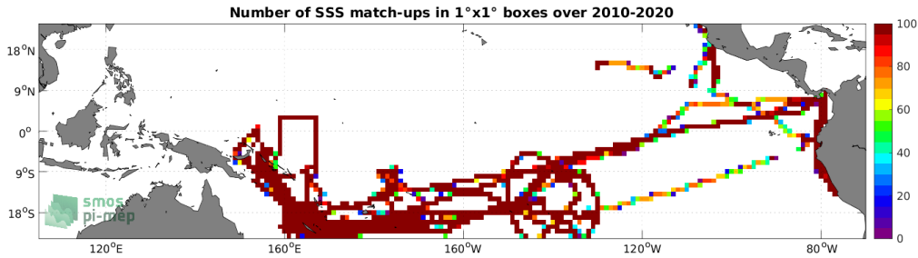
Figure 4: Number of SSS match-ups between TSG (GOSUD-Research-vessel) SSS and the SMOS SSS L3 v8 - 9 Days (CATDS-CECOS-LOCEAN) SSS product for the Tropical Pacific Ocean Pi-MEP region over 1^\circ \times 1^\circ boxes and for the full satellite product period.
