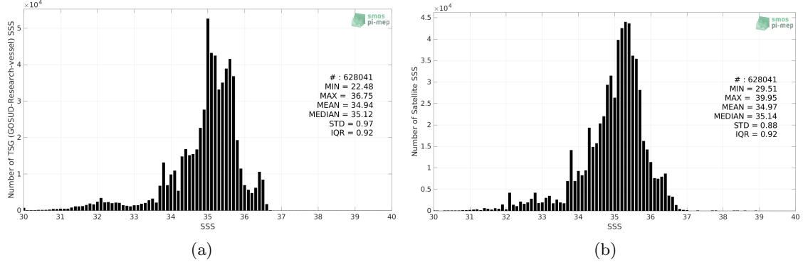
Figure 2: Histograms of SSS from TSG (GOSUD-Research-vessel) (a) and SMOS SSS L3 v8 - 9 Days (CATDS-CECOS-LOCEAN) (b) considering all match-up pairs per bins of 0.1 over the Tropical Pacific Ocean Pi-MEP region and for the full satellite product period.
