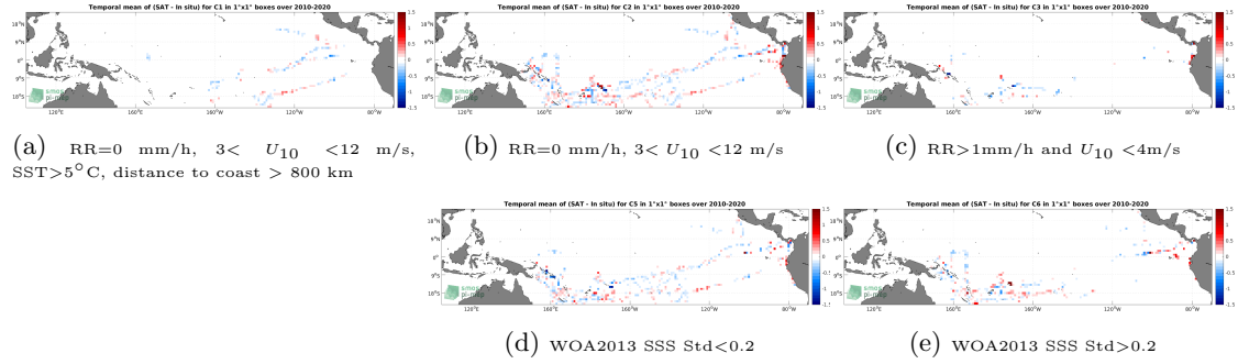
Figure 12: Temporal mean gridded over spatial boxes of size 1^{\circ}\times 1^{\circ} of \Delta SSS (SMOS SSS L3 v8 - 9 Days (CATDS-CECOS-LOCEAN) - TSG (GOSUD-Research-vessel)) for 5 different subdatasets corresponding to: RR=0 mm/h, 3 < U_{10} < 12 m/s, SST > 5^{\circ}\text{C} , distance to coast > 800 km (a), RR=0 mm/h, 3 < U_{10} < 12 m/s (b), RR > 1 mm/h and U_{10} < 4 m/s (c), WOA2013 SSS Std < 0.2 (d), WOA2013 SSS Std > 0.2 (e).
