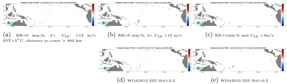
Figure 12: Temporal mean gridded over spatial boxes of size 1^{\circ}\times 1^{\circ} of \Delta\text{SSS} (SMOS SSS L3 v8 - 9 Days (CATDS-CEC-LOCEAN) - TSG (CSIC-UTM)) for 5 different subdatasets corresponding to:RR=0 mm/h, 3 < U_{10} < 12 m/s, SST >5^{\circ}\text{C} , distance to coast > 800 km (a), RR=0 mm/h, 3 < U_{10} < 12 m/s (b), RR >1 mm/h and U_{10} < 4 m/s (c), WOA2013 SSS Std <0.2 (d), WOA2013 SSS Std >0.2 (e).
