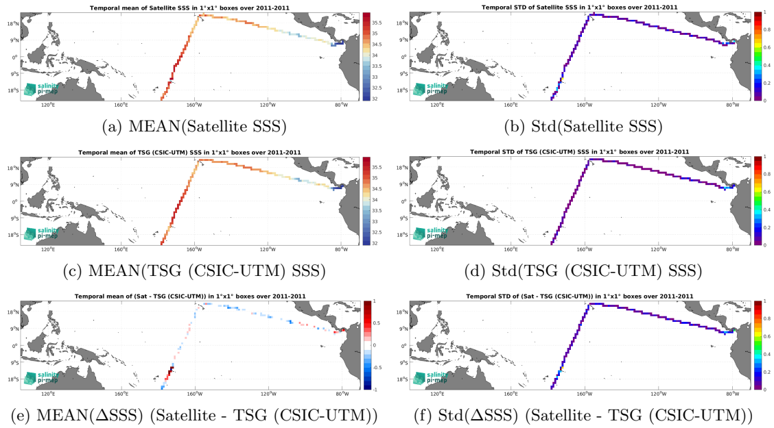
Figure 6: Temporal mean (left) and Std (right) of SSS from SMOS SSS L3 v8 - 9 Days (CATDS-CEC-LOCEAN) (top), TSG (CSIC-UTM) (middle), and of \Delta SSS (Satellite - TSG (CSIC-UTM)). Only match-up pairs are used to generate these maps.
