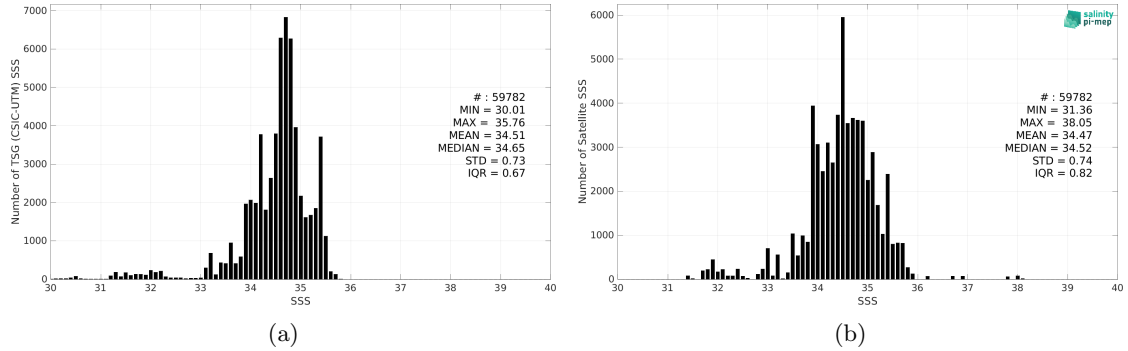
Figure 2: Histograms of SSS from TSG (CSIC-UTM) (a) and SMOS SSS L3 v8 - 9 Days (CATDS-CEC-LOCEAN) (b) considering all match-up pairs per bins of 0.1 over the Tropical Pacific Ocean Pi-MEP region and for the full satellite product period.
