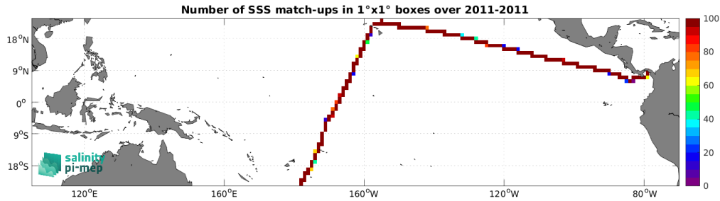
Figure 4: Number of SSS match-ups between TSG (CSIC-UTM) SSS and the SMOS SSS L3 v8 - 9 Days (CATDS-CEC-LOCEAN) SSS product for the Tropical Pacific Ocean Pi-MEP region over 1^\circ \times 1^\circ boxes and for the full satellite product period.
