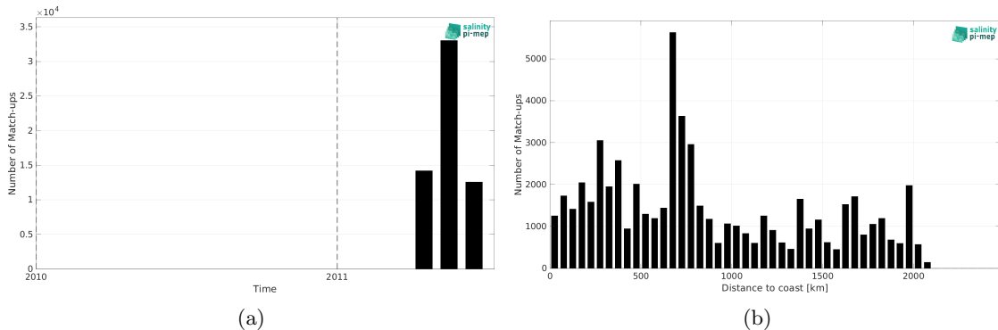
Figure 1: Number of match-ups between TSG (CSIC-UTM) and SMOS SSS L3 v8 - 9 Days (CATDS-CEC-LOCEAN) SSS as a function of time (a) and as function of the distance to coast (b) over the Tropical Pacific Ocean Pi-MEP region and for the full satellite product period.
