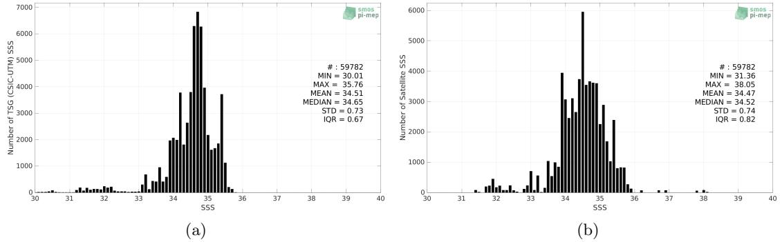
Figure 2: Histograms of SSS from TSG (CSIC-UTM) (a) and SMOS SSS L3 v8 - 9 Days (CATDS-CECOS-LOCEAN) (b) considering all match-up pairs per bins of 0.1 over the Tropical Pacific Ocean Pi-MEP region and for the full satellite product period.
