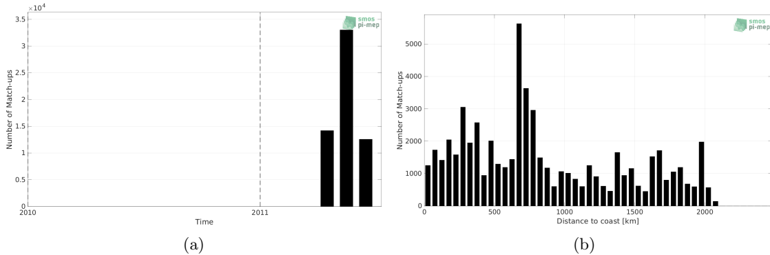
Figure 1: Number of match-ups between TSG (CSIC-UTM) and SMOS SSS L3 v8 - 9 Days (CATDS-CECOS-LOCEAN) SSS as a function of time (a) and as function of the distance to coast (b) over the Tropical Pacific Ocean Pi-MEP region and for the full satellite product period.
