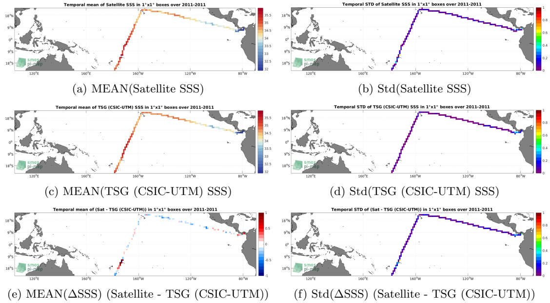
Figure 6: Temporal mean (left) and Std (right) of SSS from SMOS SSS L3 v8 - 9 Days (CATDS-CECOS-LOCEAN) (top), TSG (CSIC-UTM) (middle), and of \Delta SSS (Satellite - TSG (CSIC-UTM)). Only match-up pairs are used to generate these maps.
