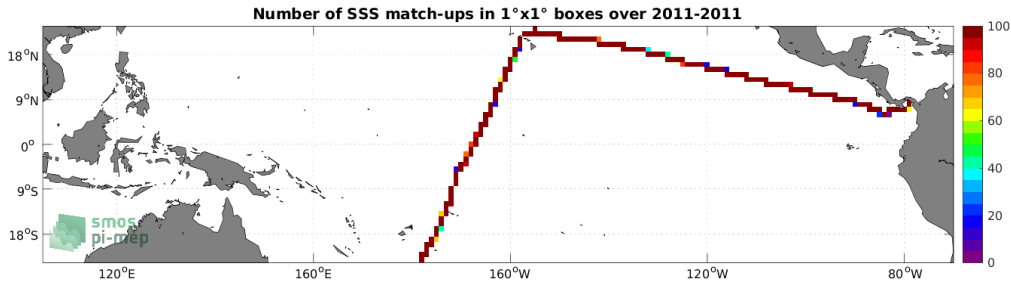
Figure 4: Number of SSS match-ups between TSG (CSIC-UTM) SSS and the SMOS SSS L3 v8 - 9 Days (CATDS-CECOS-LOCEAN) SSS product for the Tropical Pacific Ocean Pi-MEP region over 1^\circ \times 1^\circ boxes and for the full satellite product period.
