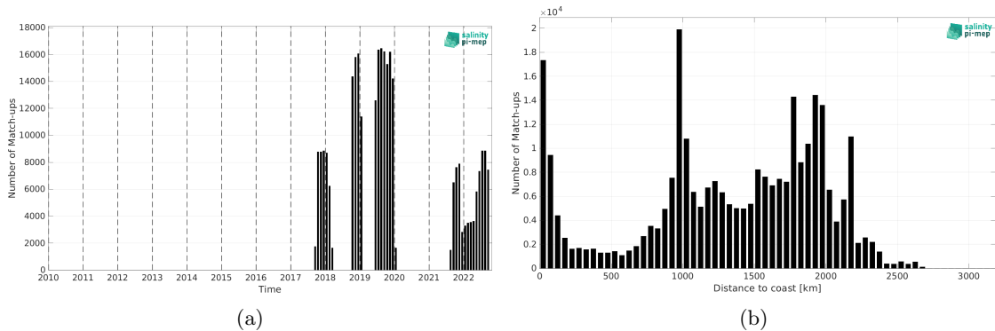
Figure 1: Number of match-ups between Saildrone and SMOS SSS L3 v8 - 9 Days (CATDS-CEC-LOCEAN) SSS as a function of time (a) and as function of the distance to coast (b) over the Tropical Pacific Ocean Pi-MEP region and for the full satellite product period.
