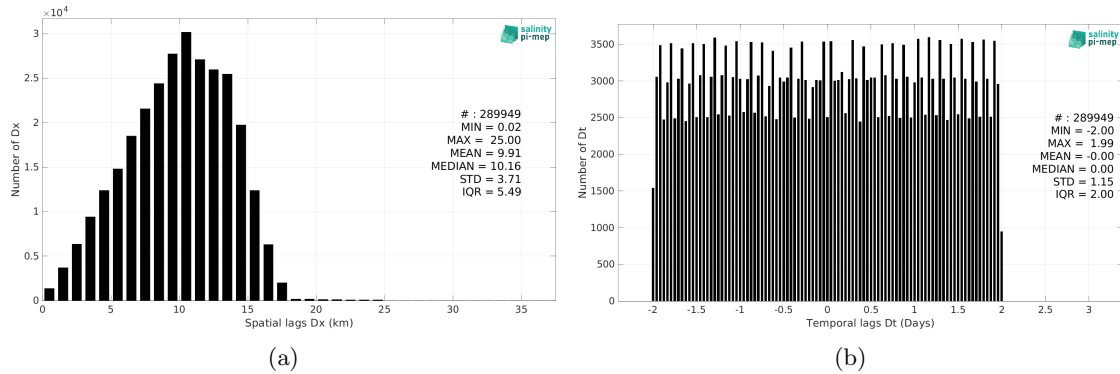
Figure 5: Histograms of the spatial (a) and temporal (b) lags between the location/time of the Saildrone measurement and the date of the corresponding SMOS SSS L3 v8 - 9 Days (CATDS-CEC-LOCEAN) SSS pixel.
