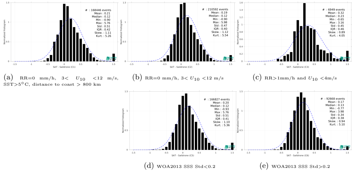
Figure 13: Normalized histogram of \Delta SSS (SMOS SSS L3 v8 - 9 Days (CATDS-CEC-LOCEAN) - Saildrone) for 5 different subdatasets corresponding to: RR=0 mm/h, 3 < U_{10} < 12 m/s, SST>5°C, distance to coast > 800 km (a), RR=0 mm/h, 3 < U_{10} < 12 m/s (b), RR>1mm/h and U_{10} < 4 m/s (c), WOA2013 SSS Std<0.2 (d), WOA2013 SSS Std>0.2 (e).
