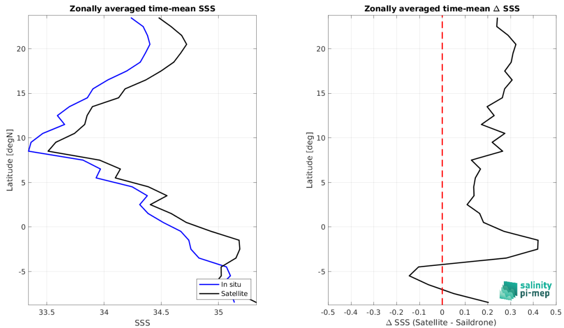
Figure 8: Left panel: Zonal mean SSS from SMOS SSS L3 v8 - 9 Days (CATDS-CEC-LOCEAN) satellite product (black) and from Saildrone (blue). Right panel: Zonal mean of \Delta SSS (Satellite - Saildrone) for all the collected Pi-MEP match-up pairs estimated over the full satellite product period.
