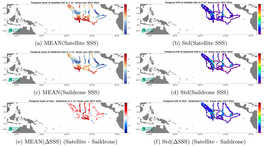
Figure 6: Temporal mean (left) and Std (right) of SSS from SMOS SSS L3 v8 - 9 Days (CATDS-CEC-LOCEAN) (top), Saildrone (middle), and of \Delta SSS (Satellite - Saildrone). Only match-up pairs are used to generate these maps.
