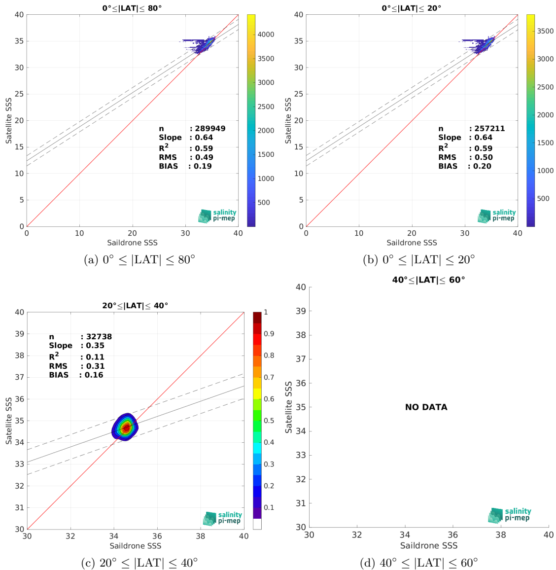
Figure 9: Contour maps of the concentration of SMOS SSS L3 v8 - 9 Days (CATDS-CEC-LOCEAN) SSS (y-axis) versus Sairdrone SSS (x-axis) at match-up pairs for different latitude bands. For each plot, the red line shows x=y . The black thin and dashed lines indicate a linear fit through the data cloud and the \pm 95\% confidence levels, respectively. The number match-up pairs n , the slope and R^2 coefficient of the linear fit, the root mean square (RMS) and the mean bias between satellite and in situ data are indicated for each latitude band in each plots.
