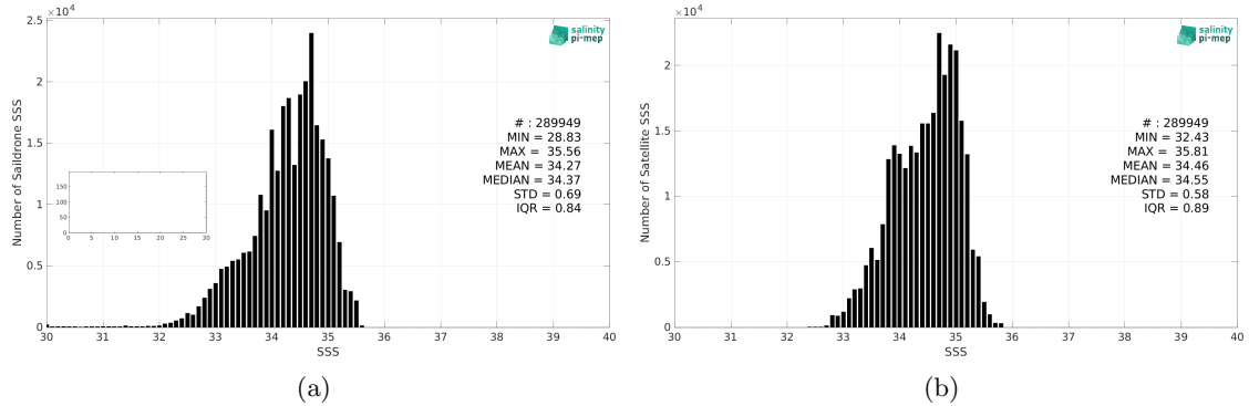
Figure 2: Histograms of SSS from Saildrone (a) and SMOS SSS L3 v8 - 9 Days (CATDS-CEC-LOCEAN) (b) considering all match-up pairs per bins of 0.1 over the Tropical Pacific Ocean Pi-MEP region and for the full satellite product period.
