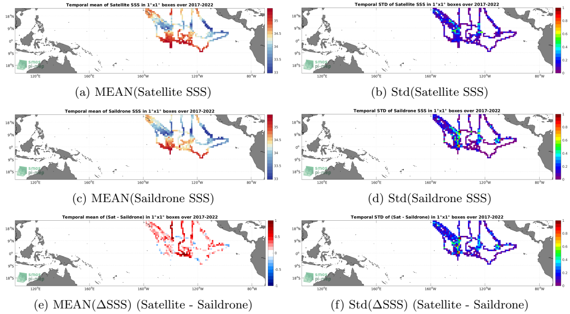
Figure 6: Temporal mean (left) and Std (right) of SSS from SMOS SSS L3 v8 - 9 Days (CATDS-CECOS-LOCEAN) (top), Saildrone (middle), and of \Delta SSS (Satellite - Saildrone). Only match-up pairs are used to generate these maps.
