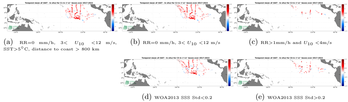
Figure 12: Temporal mean gridded over spatial boxes of size 1^\circ \times 1^\circ of \Delta SSS (SMOS SSS L3 v8 - 9 Days (CATDS-CECOS-LOCEAN) - Saildrone) for 5 different subdatasets corresponding to: RR=0 mm/h, 3 < U_{10} < 12 m/s, SST > 5^\circ\text{C} , distance to coast > 800 km (a), RR=0 mm/h, 3 < U_{10} < 12 m/s (b), RR > 1 mm/h and U_{10} < 4 m/s (c), WOA2013 SSS Std < 0.2 (d), WOA2013 SSS Std > 0.2 (e).
