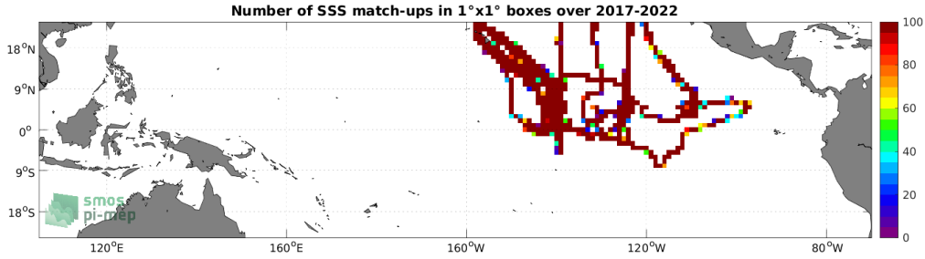
Figure 4: Number of SSS match-ups between Saildrone SSS and the SMOS SSS L3 v8 - 9 Days (CATDS-CECOS-LOCEAN) SSS product for the Tropical Pacific Ocean Pi-MEP region over 1^\circ \times 1^\circ boxes and for the full satellite product period.
