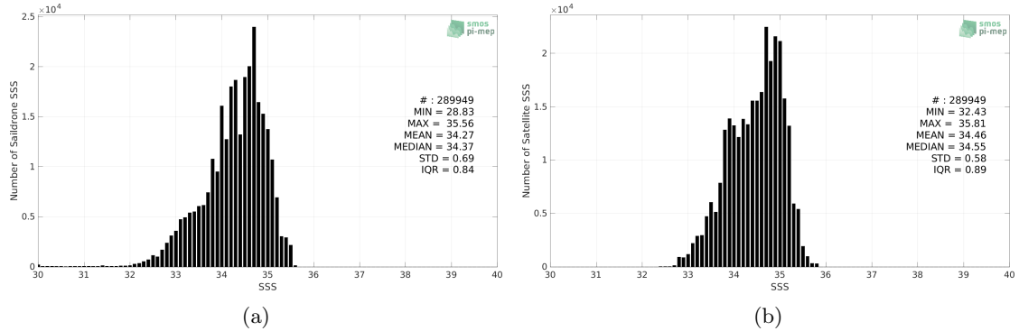
Figure 2: Histograms of SSS from Saildrone (a) and SMOS SSS L3 v8 - 9 Days (CATDS-CECOS-LOCEAN) (b) considering all match-up pairs per bins of 0.1 over the Tropical Pacific Ocean Pi-MEP region and for the full satellite product period.
