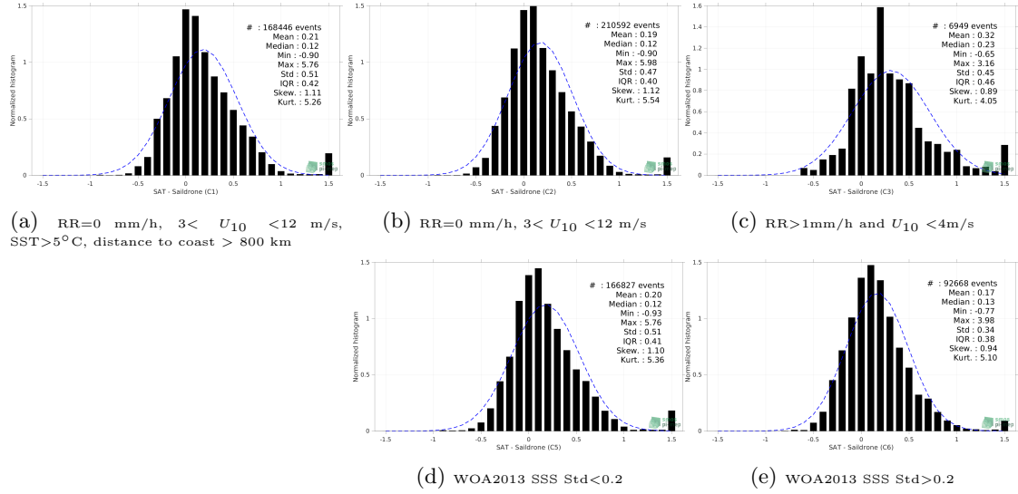
Figure 13: Normalized histogram of \Delta SSS (SMOS SSS L3 v8 - 9 Days (CATDS-CECOS-LOCEAN) - Saildrone) for 5 different subdatasets corresponding to: RR=0 mm/h, 3 < U_{10} < 12 m/s, SST>5°C, distance to coast > 800 km (a), RR=0 mm/h, 3 < U_{10} < 12 m/s (b), RR>1mm/h and U_{10} < 4 m/s (c), WOA2013 SSS Std<0.2 (d), WOA2013 SSS Std>0.2 (e).
