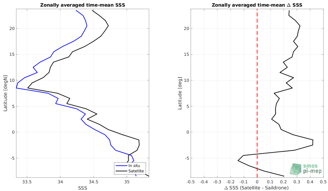
Figure 8: Left panel: Zonal mean SSS from SMOS SSS L3 v8 - 9 Days (CATDS-CECOS-LOCEAN) satellite product (black) and from Saildrone (blue). Right panel: Zonal mean of \Delta SSS (Satellite - Saildrone) for all the collected Pi-MEP match-up pairs estimated over the full satellite product period.
