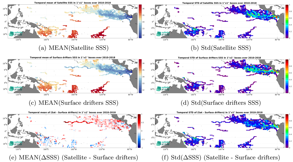
Figure 5: Temporal mean (left) and Std (right) of SSS from SMOS SSS L3 v8 - 9 Days (CATDS-CEC-LOCEAN) (top), Surface drifters (middle), and of \Delta SSS (Satellite - Surface drifters). Only match-up pairs are used to generate these maps.
