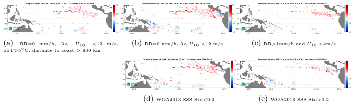
Figure 11: Temporal mean gridded over spatial boxes of size 1^\circ \times 1^\circ of \Delta SSS (SMOS SSS L3 v8 - 9 Days (CATDS-CEC-LOCEAN) - Surface drifters) for 5 different subdatasets corresponding to: RR=0 mm/h, 3 < U_{10} < 12 m/s, SST > 5^\circ\text{C} , distance to coast > 800 km (a), RR=0 mm/h, 3 < U_{10} < 12 m/s (b), RR > 1 mm/h and U_{10} < 4 m/s (c), WOA2013 SSS Std < 0.2 (d), WOA2013 SSS Std > 0.2 (e).
