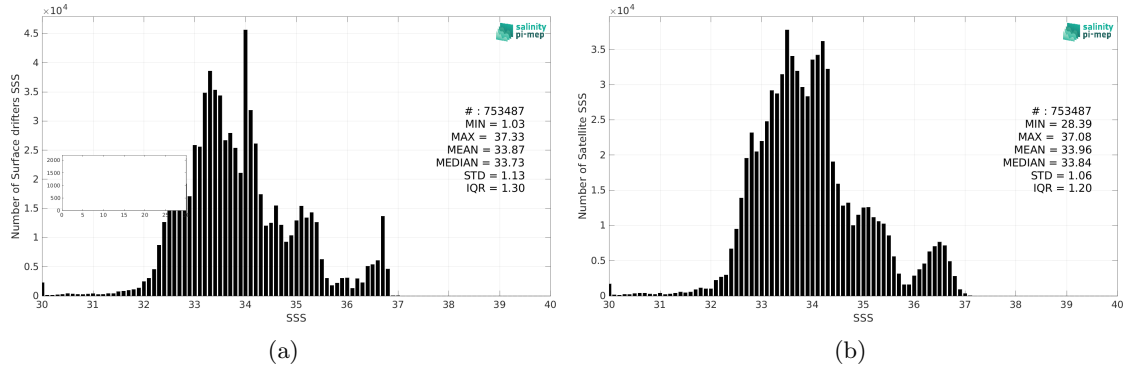
Figure 2: Histograms of SSS from Surface drifters (a) and SMOS SSS L3 v8 - 9 Days (CATDS-CEC-LOCEAN) (b) considering all match-up pairs per bins of 0.1 over the Tropical Pacific Ocean Pi-MEP region and for the full satellite product period.
