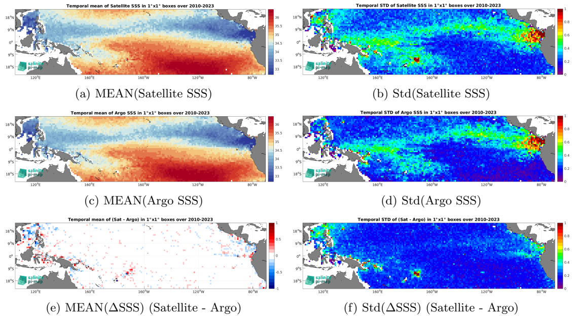
Figure 6: Temporal mean (left) and Std (right) of SSS from SMOS SSS L3 v8 - 9 Days (CATDS-CEC-LOCEAN) (top), Argo (middle), and of \Delta SSS (Satellite - Argo). Only match-up pairs are used to generate these maps.
