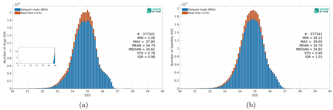
Figure 2: Histograms of SSS from Argo (a) and SMOS SSS L3 v8 - 9 Days (CATDS-CEC-LOCEAN) (b) considering all match-up pairs per bins of 0.1 over the Tropical Pacific Ocean Pi-MEP region and for the full satellite product period.
