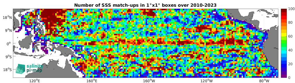
Figure 4: Number of SSS match-ups between Argo SSS and the SMOS SSS L3 v8 - 9 Days (CATDS-CEC-LOCEAN) SSS product for the Tropical Pacific Ocean Pi-MEP region over 1^\circ \times 1^\circ boxes and for the full satellite product period.
