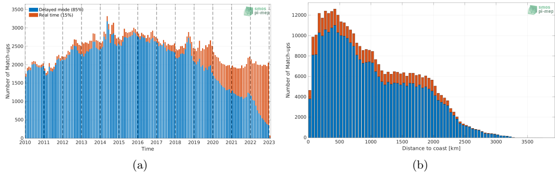
Figure 1: Number of match-ups between Argo and SMOS SSS L3 v8 - 9 Days (CATDS-CECOS-LOCEAN) SSS as a function of time (a) and as function of the distance to coast (b) over the Tropical Pacific Ocean Pi-MEP region and for the full satellite product period.
