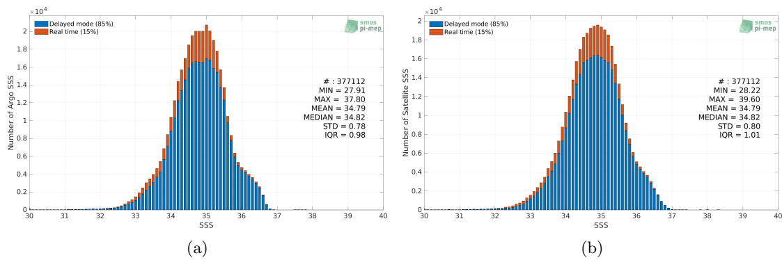
Figure 2: Histograms of SSS from Argo (a) and SMOS SSS L3 v8 - 9 Days (CATDS-CECOS-LOCEAN) (b) considering all match-up pairs per bins of 0.1 over the Tropical Pacific Ocean Pi-MEP region and for the full satellite product period.
