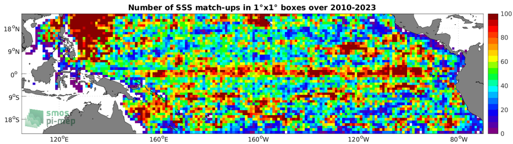
Figure 4: Number of SSS match-ups between Argo SSS and the SMOS SSS L3 v8 - 9 Days (CATDS-CECOS-LOCEAN) SSS product for the Tropical Pacific Ocean Pi-MEP region over 1^\circ \times 1^\circ boxes and for the full satellite product period.
