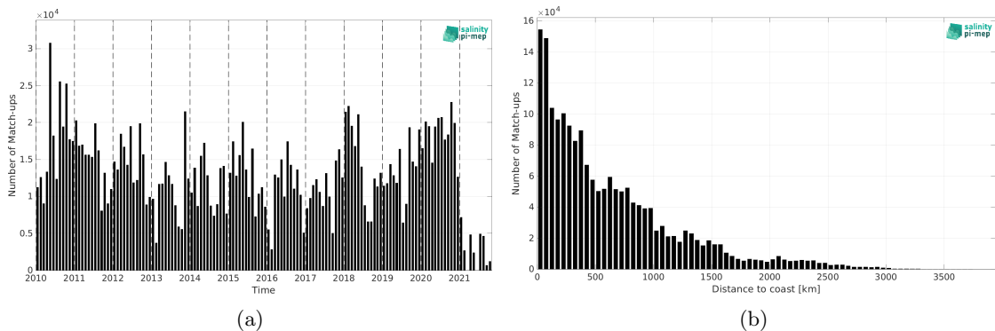
Figure 1: Number of match-ups between TSG (LEGOS-DM) and SMOS SSS L3 v8 - 18 Days (CATDS-CEC-LOCEAN) SSS as a function of time (a) and as function of the distance to coast (b) over the Tropical Pacific Ocean Pi-MEP region and for the full satellite product period.
