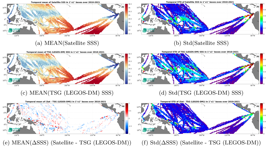
Figure 6: Temporal mean (left) and Std (right) of SSS from SMOS SSS L3 v8 - 18 Days (CATDS-CEC-LOCEAN) (top), TSG (LEGOS-DM) (middle), and of \Delta SSS (Satellite - TSG (LEGOS-DM)). Only match-up pairs are used to generate these maps.
