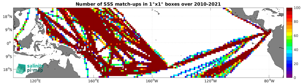
Figure 4: Number of SSS match-ups between TSG (LEGOS-DM) SSS and the SMOS SSS L3 v8 - 18 Days (CATDS-CEC-LOCEAN) SSS product for the Tropical Pacific Ocean Pi-MEP region over 1^\circ \times 1^\circ boxes and for the full satellite product period.
