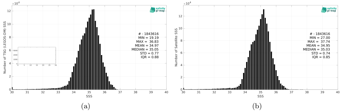
Figure 2: Histograms of SSS from TSG (LEGOS-DM) (a) and SMOS SSS L3 v8 - 18 Days (CATDS-CEC-LOCEAN) (b) considering all match-up pairs per bins of 0.1 over the Tropical Pacific Ocean Pi-MEP region and for the full satellite product period.
