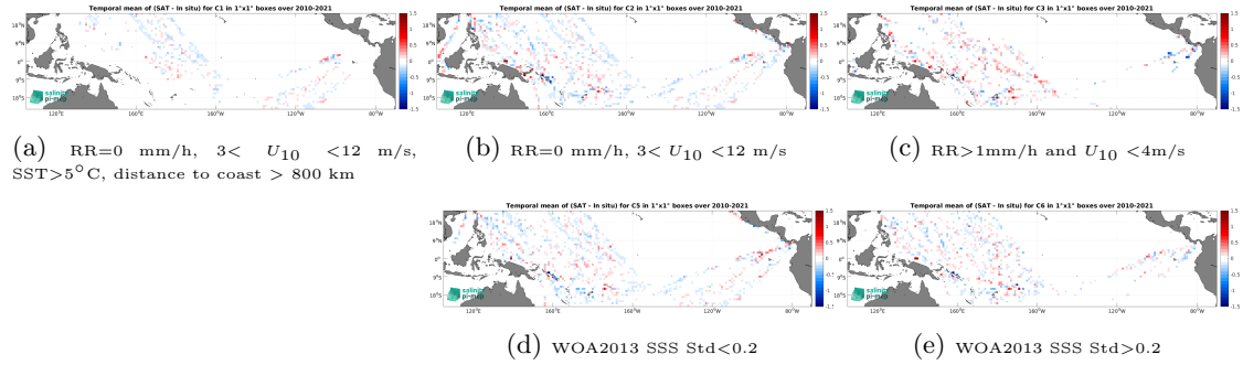
Figure 12: Temporal mean gridded over spatial boxes of size 1^{\circ}\times 1^{\circ} of \Delta\text{SSS} (SMOS SSS L3 v8 - 18 Days (CATDS-CEC-LOCEAN) - TSG (LEGOS-DM)) for 5 different subdatasets corresponding to:RR=0 mm/h, 3 < U_{10} < 12 m/s, SST > 5^{\circ}\text{C} , distance to coast > 800 km (a), RR=0 mm/h, 3 < U_{10} < 12 m/s (b), RR > 1 mm/h and U_{10} < 4 m/s (c), WOA2013 SSS Std < 0.2 (d), WOA2013 SSS Std > 0.2 (e).
