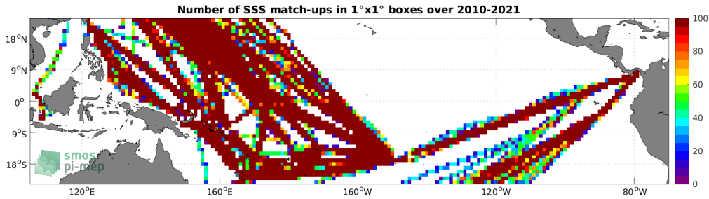
Figure 4: Number of SSS match-ups between TSG (LEGOS-DM) SSS and the SMOS SSS L3 v8 - 18 Days (CATDS-CECOS-LOCEAN) SSS product for the Tropical Pacific Ocean Pi-MEP region over 1^\circ \times 1^\circ boxes and for the full satellite product period.
