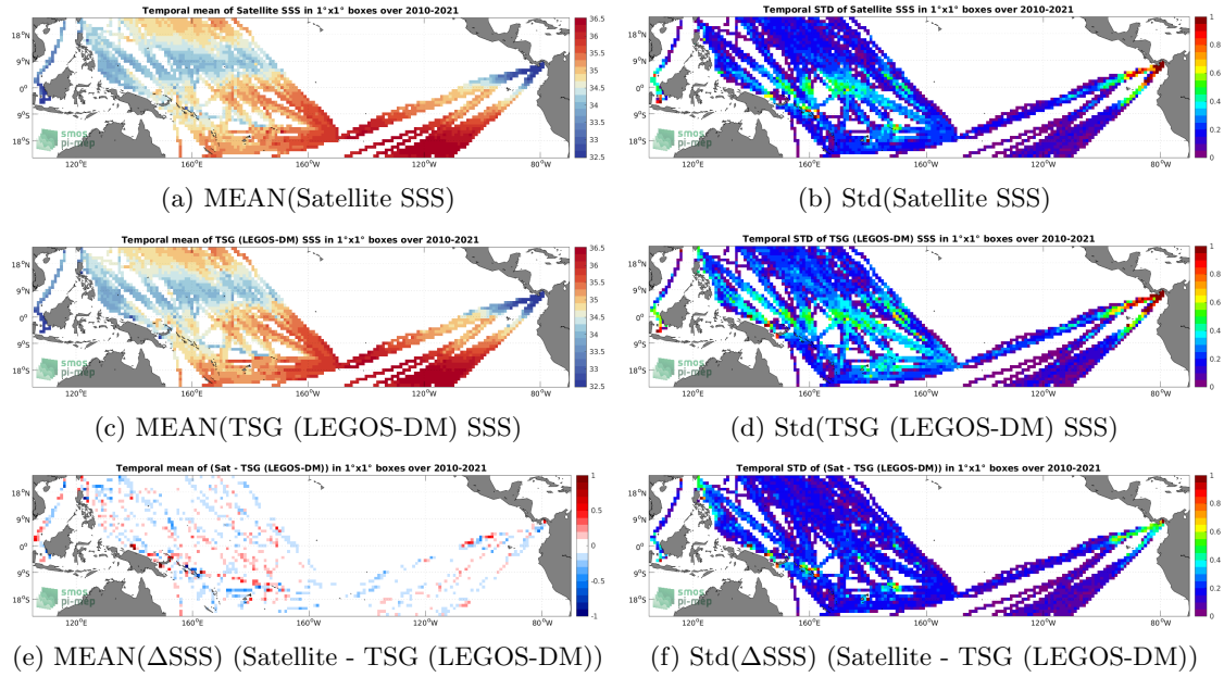
Figure 6: Temporal mean (left) and Std (right) of SSS from SMOS SSS L3 v8 - 18 Days (CATDS-CECOS-LOCEAN) (top), TSG (LEGOS-DM) (middle), and of \Delta SSS (Satellite - TSG (LEGOS-DM)). Only match-up pairs are used to generate these maps.
