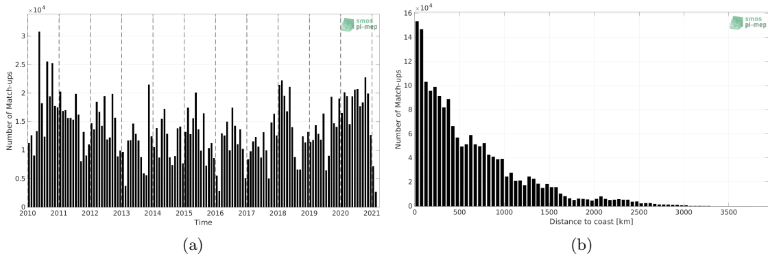
Figure 1: Number of match-ups between TSG (LEGOS-DM) and SMOS SSS L3 v8 - 18 Days (CATDS-CECOS-LOCEAN) SSS as a function of time (a) and as function of the distance to coast (b) over the Tropical Pacific Ocean Pi-MEP region and for the full satellite product period.
