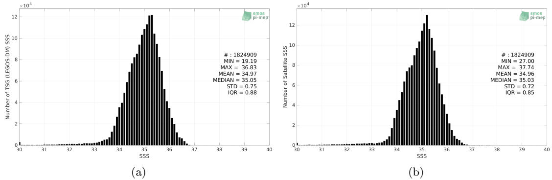
Figure 2: Histograms of SSS from TSG (LEGOS-DM) (a) and SMOS SSS L3 v8 - 18 Days (CATDS-CECOS-LOCEAN) (b) considering all match-up pairs per bins of 0.1 over the Tropical Pacific Ocean Pi-MEP region and for the full satellite product period.
