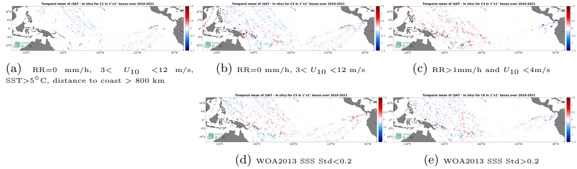
Figure 12: Temporal mean gridded over spatial boxes of size 1^{\circ}\times 1^{\circ} of \Delta\text{SSS} (SMOS SSS L3 v8 - 18 Days (CATDS-CECOS-LOCEAN) - TSG (LEGOS-DM)) for 5 different subdatasets corresponding to:RR=0 mm/h, 3 < U_{10} < 12 m/s, SST > 5^{\circ}\text{C} , distance to coast > 800 km (a), RR=0 mm/h, 3 < U_{10} < 12 m/s (b), RR > 1 mm/h and U_{10} < 4 m/s (c), WOA2013 SSS Std < 0.2 (d), WOA2013 SSS Std > 0.2 (e).
