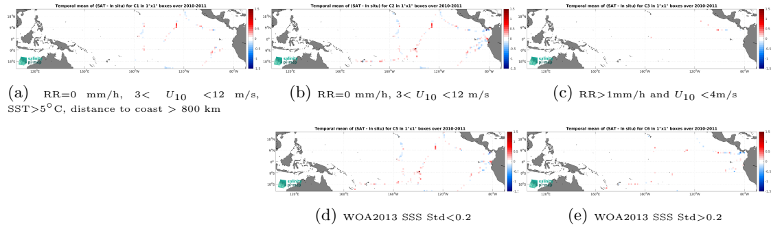
Figure 12: Temporal mean gridded over spatial boxes of size 1^{\circ}\times 1^{\circ} of \Delta SSS (SMOS SSS L3 v8 - 18 Days (CATDS-CEC-LOCEAN) - TSG (GOSUD-Sailing-ship)) for 5 different subdatasets corresponding to:RR=0 mm/h, 3 < U_{10} < 12 m/s, SST >5^{\circ}\text{C} , distance to coast > 800 km (a), RR=0 mm/h, 3 < U_{10} < 12 m/s (b), RR >1 mm/h and U_{10} < 4 m/s (c), WOA2013 SSS Std <0.2 (d), WOA2013 SSS Std >0.2 (e).
