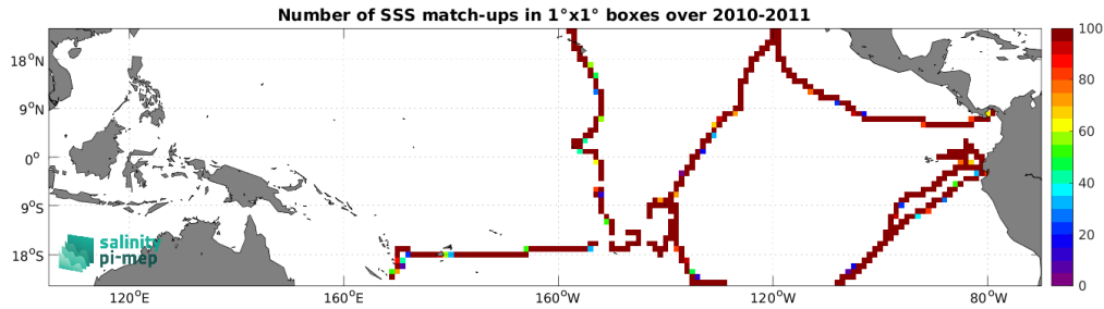
Figure 4: Number of SSS match-ups between TSG (GOSUD-Sailing-ship) SSS and the SMOS SSS L3 v8 - 18 Days (CATDS-CEC-LOCEAN) SSS product for the Tropical Pacific Ocean Pi-MEP region over 1^\circ \times 1^\circ boxes and for the full satellite product period.
