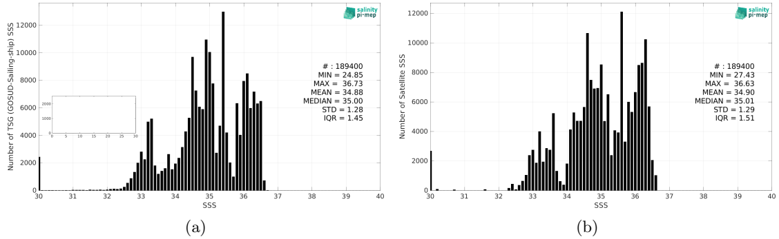
Figure 2: Histograms of SSS from TSG (GOSUD-Sailing-ship) (a) and SMOS SSS L3 v8 - 18 Days (CATDS-CEC-LOCEAN) (b) considering all match-up pairs per bins of 0.1 over the Tropical Pacific Ocean Pi-MEP region and for the full satellite product period.
