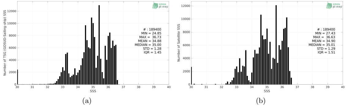
Figure 2: Histograms of SSS from TSG (GOSUD-Sailing-ship) (a) and SMOS SSS L3 v8 - 18 Days (CATDS-CECOS-LOCEAN) (b) considering all match-up pairs per bins of 0.1 over the Tropical Pacific Ocean Pi-MEP region and for the full satellite product period.
