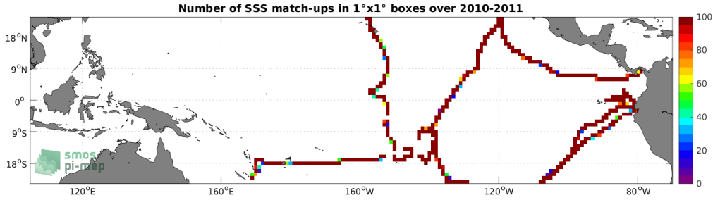
Figure 4: Number of SSS match-ups between TSG (GOSUD-Sailing-ship) SSS and the SMOS SSS L3 v8 - 18 Days (CATDS-CECOS-LOCEAN) SSS product for the Tropical Pacific Ocean Pi-MEP region over 1^\circ \times 1^\circ boxes and for the full satellite product period.
