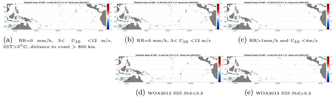
Figure 12: Temporal mean gridded over spatial boxes of size 1^{\circ}\times 1^{\circ} of \Delta SSS (SMOS SSS L3 v8 - 18 Days (CATDS-CECOS-LOCEAN) - TSG (GOSUD-Sailing-ship)) for 5 different subdatasets corresponding to:RR=0 mm/h, 3 < U_{10} < 12 m/s, SST >5^{\circ}\text{C} , distance to coast > 800 km (a), RR=0 mm/h, 3 < U_{10} < 12 m/s (b), RR >1 mm/h and U_{10} < 4 m/s (c), WOA2013 SSS Std <0.2 (d), WOA2013 SSS Std >0.2 (e).
