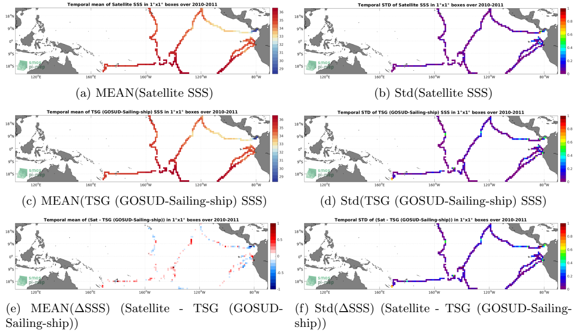
Figure 6: Temporal mean (left) and Std (right) of SSS from SMOS SSS L3 v8 - 18 Days (CATDS-CECOS-LOCEAN) (top), TSG (GOSUD-Sailing-ship) (middle), and of \Delta SSS (Satellite - TSG (GOSUD-Sailing-ship)). Only match-up pairs are used to generate these maps.
