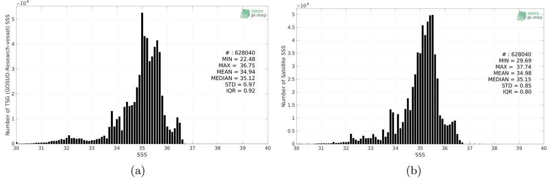
Figure 2: Histograms of SSS from TSG (GOSUD-Research-vessel) (a) and SMOS SSS L3 v8 - 18 Days (CATDS-CECOS-LOCEAN) (b) considering all match-up pairs per bins of 0.1 over the Tropical Pacific Ocean Pi-MEP region and for the full satellite product period.
