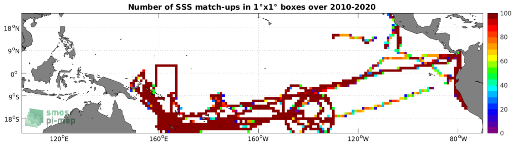
Figure 4: Number of SSS match-ups between TSG (GOSUD-Research-vessel) SSS and the SMOS SSS L3 v8 - 18 Days (CATDS-CECOS-LOCEAN) SSS product for the Tropical Pacific Ocean Pi-MEP region over 1^\circ \times 1^\circ boxes and for the full satellite product period.
