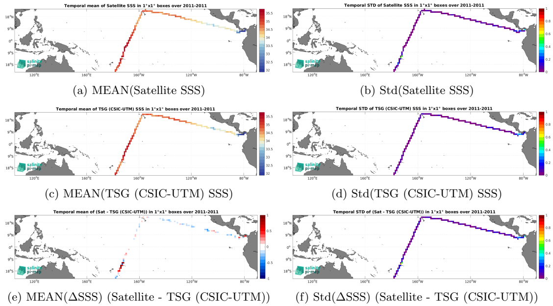
Figure 6: Temporal mean (left) and Std (right) of SSS from SMOS SSS L3 v8 - 18 Days (CATDS-CEC-LOCEAN) (top), TSG (CSIC-UTM) (middle), and of \Delta SSS (Satellite - TSG (CSIC-UTM)). Only match-up pairs are used to generate these maps.
