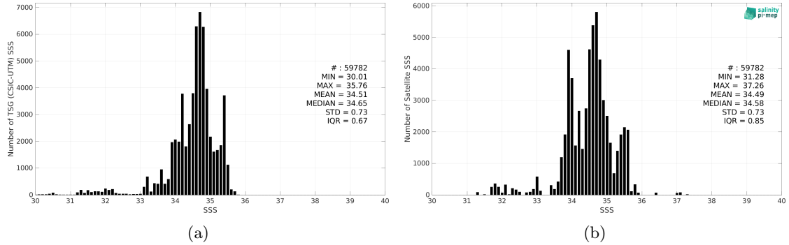
Figure 2: Histograms of SSS from TSG (CSIC-UTM) (a) and SMOS SSS L3 v8 - 18 Days (CATDS-CEC-LOCEAN) (b) considering all match-up pairs per bins of 0.1 over the Tropical Pacific Ocean Pi-MEP region and for the full satellite product period.
