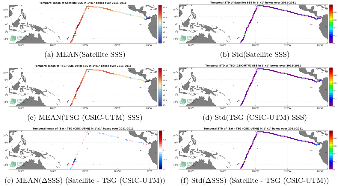
Figure 6: Temporal mean (left) and Std (right) of SSS from SMOS SSS L3 v8 - 18 Days (CATDS-CECOS-LOCEAN) (top), TSG (CSIC-UTM) (middle), and of \Delta SSS (Satellite - TSG (CSIC-UTM)). Only match-up pairs are used to generate these maps.
