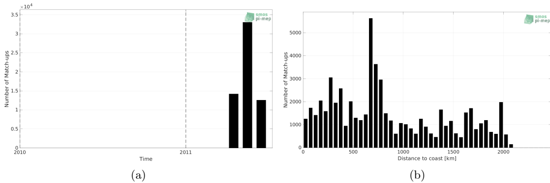
Figure 1: Number of match-ups between TSG (CSIC-UTM) and SMOS SSS L3 v8 - 18 Days (CATDS-CECOS-LOCEAN) SSS as a function of time (a) and as function of the distance to coast (b) over the Tropical Pacific Ocean Pi-MEP region and for the full satellite product period.
