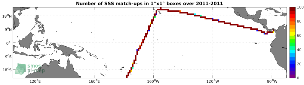
Figure 4: Number of SSS match-ups between TSG (CSIC-UTM) SSS and the SMOS SSS L3 v8 - 18 Days (CATDS-CECOS-LOCEAN) SSS product for the Tropical Pacific Ocean Pi-MEP region over 1^\circ \times 1^\circ boxes and for the full satellite product period.
