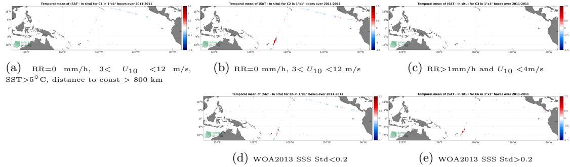
Figure 12: Temporal mean gridded over spatial boxes of size 1^{\circ}\times 1^{\circ} of \Delta\text{SSS} (SMOS SSS L3 v8 - 18 Days (CATDS-CECOS-LOCEAN) - TSG (CSIC-UTM)) for 5 different subdatasets corresponding to:RR=0 mm/h, 3 < U_{10} < 12 m/s, SST >5^{\circ}\text{C} , distance to coast > 800 km (a), RR=0 mm/h, 3 < U_{10} < 12 m/s (b), RR >1 mm/h and U_{10} < 4 m/s (c), WOA2013 SSS Std <0.2 (d), WOA2013 SSS Std >0.2 (e).
