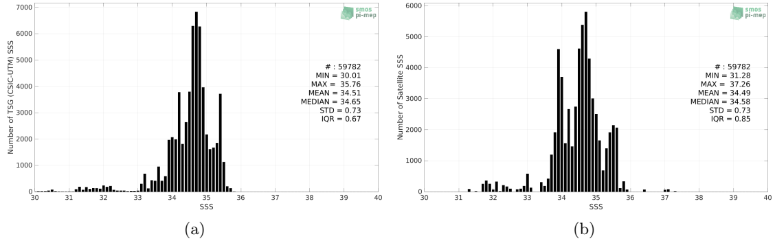
Figure 2: Histograms of SSS from TSG (CSIC-UTM) (a) and SMOS SSS L3 v8 - 18 Days (CATDS-CECOS-LOCEAN) (b) considering all match-up pairs per bins of 0.1 over the Tropical Pacific Ocean Pi-MEP region and for the full satellite product period.
