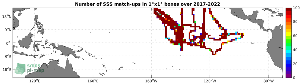
Figure 4: Number of SSS match-ups between Saildrone SSS and the SMOS SSS L3 v8 - 18 Days (CATDS-CECOS-LOCEAN) SSS product for the Tropical Pacific Ocean Pi-MEP region over 1^\circ \times 1^\circ boxes and for the full satellite product period.
