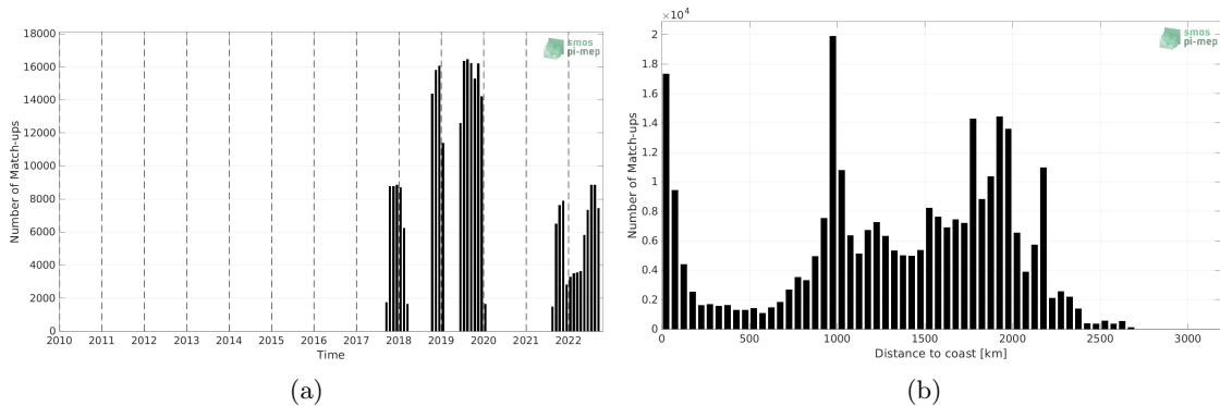
Figure 1: Number of match-ups between Saildrone and SMOS SSS L3 v8 - 18 Days (CATDS-CECOS-LOCEAN) SSS as a function of time (a) and as function of the distance to coast (b) over the Tropical Pacific Ocean Pi-MEP region and for the full satellite product period.
