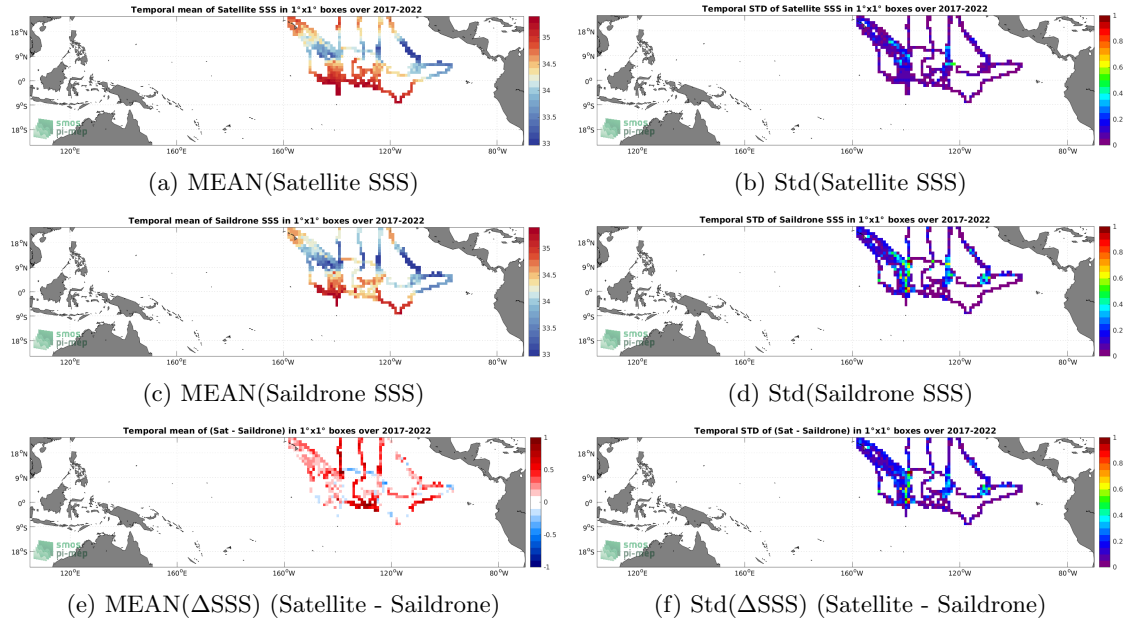
Figure 6: Temporal mean (left) and Std (right) of SSS from SMOS SSS L3 v8 - 18 Days (CATDS-CECOS-LOCEAN) (top), Saildrone (middle), and of \Delta SSS (Satellite - Saildrone). Only match-up pairs are used to generate these maps.
