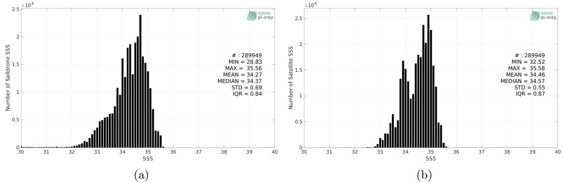
Figure 2: Histograms of SSS from Saildrone (a) and SMOS SSS L3 v8 - 18 Days (CATDS-CECOS-LOCEAN) (b) considering all match-up pairs per bins of 0.1 over the Tropical Pacific Ocean Pi-MEP region and for the full satellite product period.
