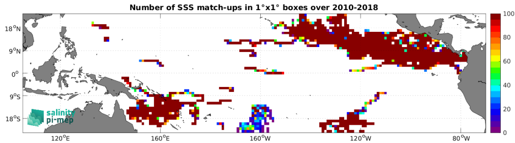
Figure 3: Number of SSS match-ups between Surface drifters SSS and the SMOS SSS L3 v8 - 18 Days (CATDS-CEC-LOCEAN) SSS product for the Tropical Pacific Ocean Pi-MEP region over 1^\circ \times 1^\circ boxes and for the full satellite product period.
