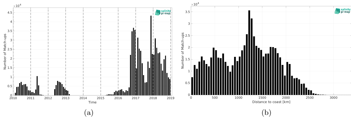
Figure 1: Number of match-ups between Surface drifters and SMOS SSS L3 v8 - 18 Days (CATDS-CEC-LOCEAN) SSS as a function of time (a) and as function of the distance to coast (b) over the Tropical Pacific Ocean Pi-MEP region and for the full satellite product period.
