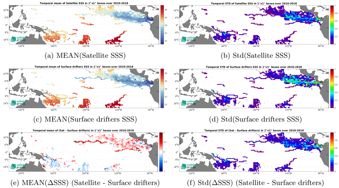
Figure 5: Temporal mean (left) and Std (right) of SSS from SMOS SSS L3 v8 - 18 Days (CATDS-CEC-LOCEAN) (top), Surface drifters (middle), and of \Delta SSS (Satellite - Surface drifters). Only match-up pairs are used to generate these maps.
