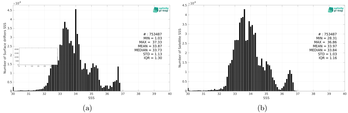
Figure 2: Histograms of SSS from Surface drifters (a) and SMOS SSS L3 v8 - 18 Days (CATDS-CEC-LOCEAN) (b) considering all match-up pairs per bins of 0.1 over the Tropical Pacific Ocean Pi-MEP region and for the full satellite product period.
