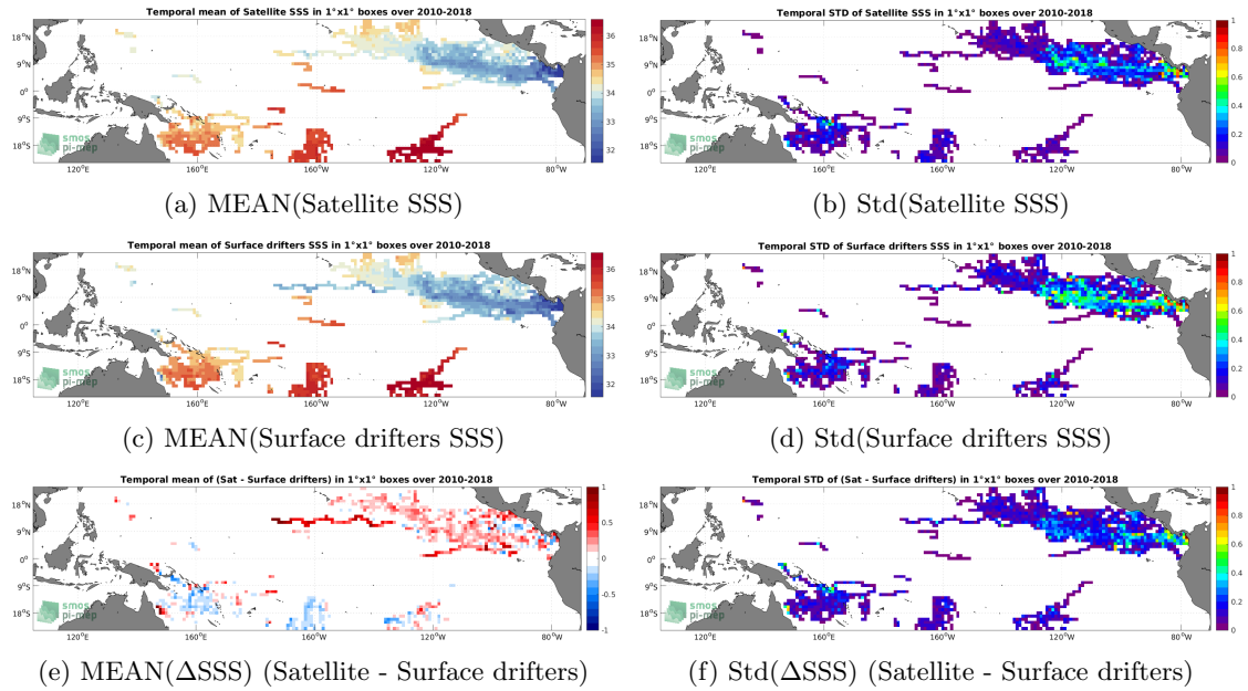
Figure 5: Temporal mean (left) and Std (right) of SSS from SMOS SSS L3 v8 - 18 Days (CATDS-CECOS-LOCEAN) (top), Surface drifters (middle), and of \Delta SSS (Satellite - Surface drifters). Only match-up pairs are used to generate these maps.
