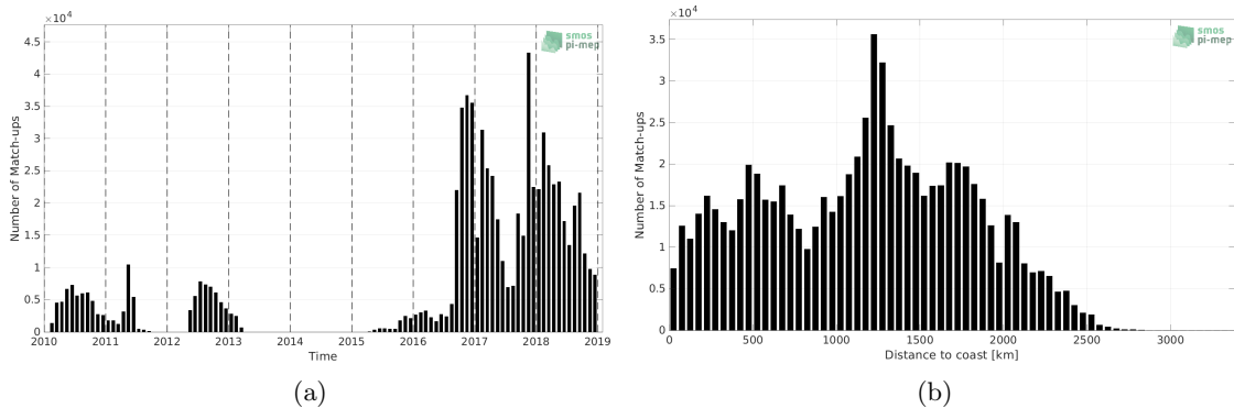
Figure 1: Number of match-ups between Surface drifters and SMOS SSS L3 v8 - 18 Days (CATDS-CECOS-LOCEAN) SSS as a function of time (a) and as function of the distance to coast (b) over the Tropical Pacific Ocean Pi-MEP region and for the full satellite product period.
