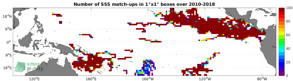
Figure 3: Number of SSS match-ups between Surface drifters SSS and the SMOS SSS L3 v8 - 18 Days (CATDS-CECOS-LOCEAN) SSS product for the Tropical Pacific Ocean Pi-MEP region over 1^\circ \times 1^\circ boxes and for the full satellite product period.
