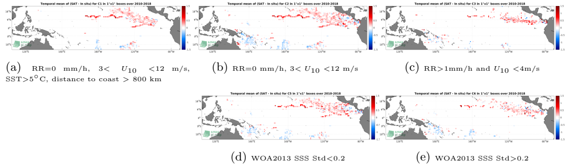
Figure 11: Temporal mean gridded over spatial boxes of size 1^{\circ}\times 1^{\circ} of \Delta\text{SSS} (SMOS SSS L3 v8 - 18 Days (CATDS-CECOS-LOCEAN) - Surface drifters) for 5 different subdatasets corresponding to:RR=0 mm/h, 3 < U_{10} < 12 m/s, SST > 5^{\circ}\text{C} , distance to coast > 800 km (a), RR=0 mm/h, 3 < U_{10} < 12 m/s (b), RR > 1 mm/h and U_{10} < 4 m/s (c), WOA2013 SSS Std < 0.2 (d), WOA2013 SSS Std > 0.2 (e).
