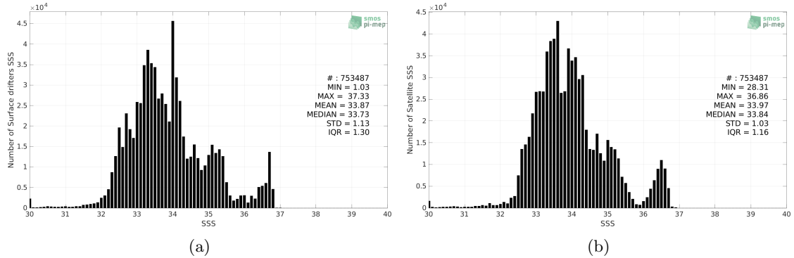
Figure 2: Histograms of SSS from Surface drifters (a) and SMOS SSS L3 v8 - 18 Days (CATDS-CECOS-LOCEAN) (b) considering all match-up pairs per bins of 0.1 over the Tropical Pacific Ocean Pi-MEP region and for the full satellite product period.
