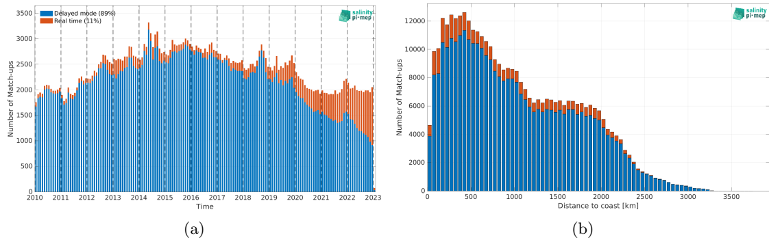
Figure 1: Number of match-ups between Argo and SMOS SSS L3 v8 - 18 Days (CATDS-CEC-LOCEAN) SSS as a function of time (a) and as function of the distance to coast (b) over the Tropical Pacific Ocean Pi-MEP region and for the full satellite product period.
