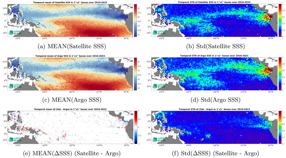
Figure 6: Temporal mean (left) and Std (right) of SSS from SMOS SSS L3 v8 - 18 Days (CATDS-CEC-LOCEAN) (top), Argo (middle), and of \Delta SSS (Satellite - Argo). Only match-up pairs are used to generate these maps.
