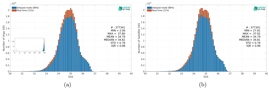
Figure 2: Histograms of SSS from Argo (a) and SMOS SSS L3 v8 - 18 Days (CATDS-CEC-LOCEAN) (b) considering all match-up pairs per bins of 0.1 over the Tropical Pacific Ocean Pi-MEP region and for the full satellite product period.
