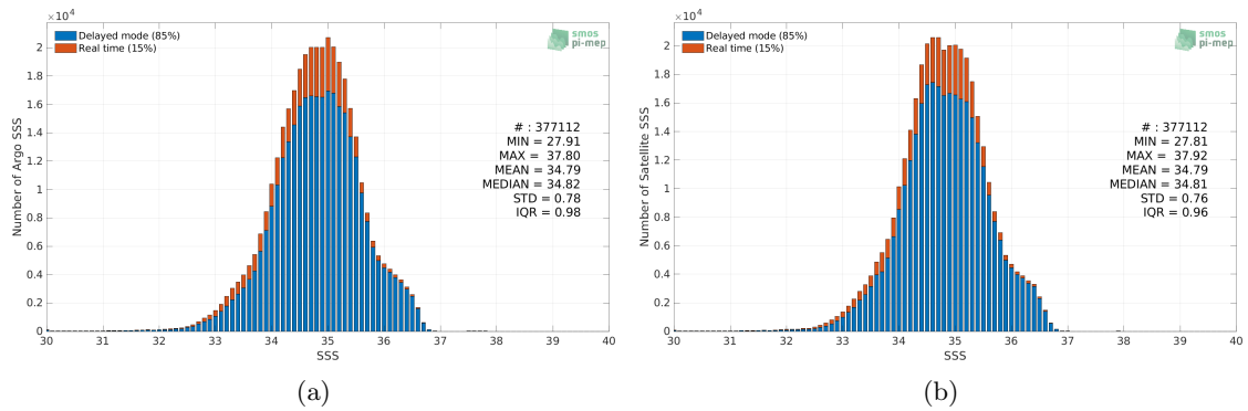
Figure 2: Histograms of SSS from Argo (a) and SMOS SSS L3 v8 - 18 Days (CATDS-CECOS-LOCEAN) (b) considering all match-up pairs per bins of 0.1 over the Tropical Pacific Ocean Pi-MEP region and for the full satellite product period.
