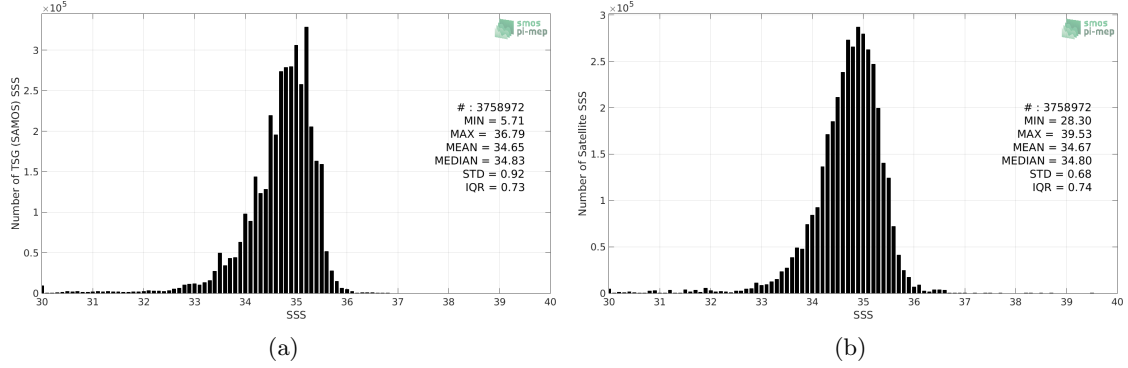
Figure 2: Histograms of SSS from TSG (SAMOS) (a) and SMOS SSS L3 v7 - 9 Days (CATDS-CECOS-LOCEAN) (b) considering all match-up pairs per bins of 0.1 over the Tropical Pacific Ocean Pi-MEP region and for the full satellite product period.
