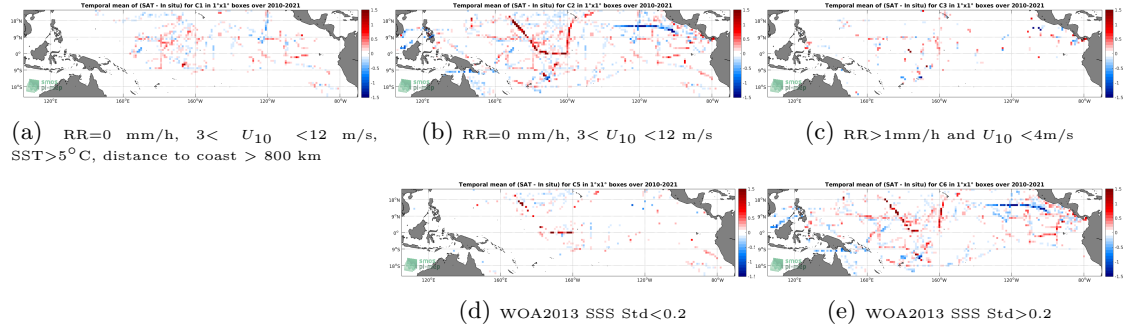
Figure 12: Temporal mean gridded over spatial boxes of size 1^{\circ} \times 1^{\circ} of \Delta\text{SSS} (SMOS SSS L3 v7 - 9 Days (CATDS-CECOS-LOCEAN) - TSG (SAMOS)) for 5 different subdatasets corresponding to:RR=0 mm/h, 3 < U_{10} < 12 m/s, SST >5^{\circ}\text{C} , distance to coast > 800 km (a), RR=0 mm/h, 3 < U_{10} < 12 m/s (b), RR >1 mm/h and U_{10} < 4 m/s (c), WOA2013 SSS Std <0.2 (d), WOA2013 SSS Std >0.2 (e).
