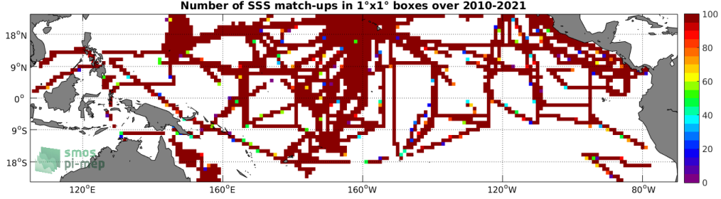
Figure 4: Number of SSS match-ups between TSG (SAMOS) SSS and the SMOS SSS L3 v7 - 9 Days (CATDS-CECOS-LOCEAN) SSS product for the Tropical Pacific Ocean Pi-MEP region over 1^\circ \times 1^\circ boxes and for the full satellite product period.
