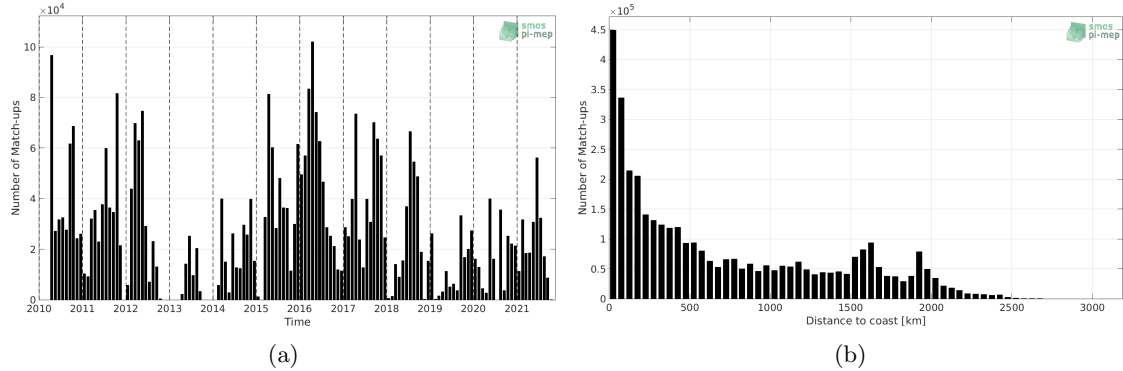
Figure 1: Number of match-ups between TSG (SAMOS) and SMOS SSS L3 v7 - 9 Days (CATDS-CECOS-LOCEAN) SSS as a function of time (a) and as function of the distance to coast (b) over the Tropical Pacific Ocean Pi-MEP region and for the full satellite product period.
