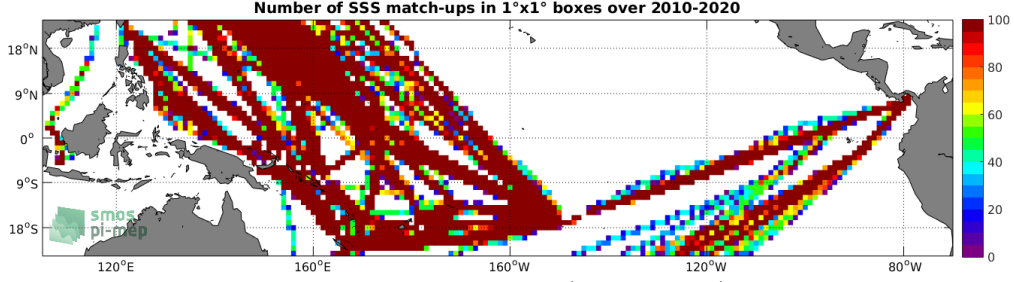
Figure 4: Number of SSS match-ups between TSG (LEGOS-DM) SSS and the SMOS SSS L3 v7 - 9 Days (CATDS-CECOS-LOCEAN) SSS product for the Tropical Pacific Ocean Pi-MEP region over 1^\circ \times 1^\circ boxes and for the full satellite product period.
