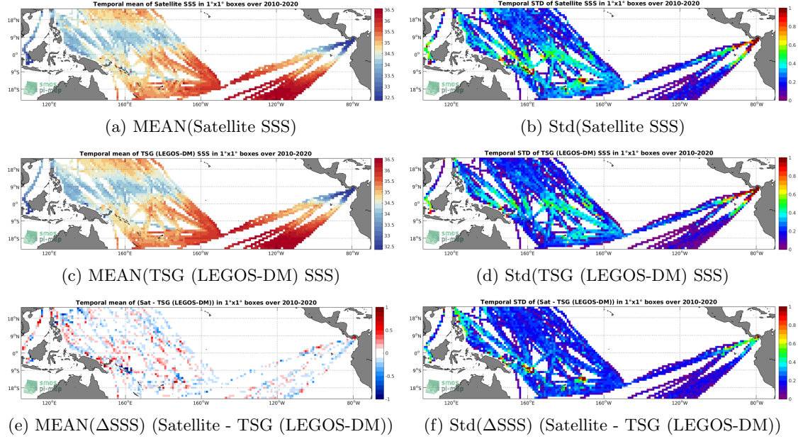
Figure 6: Temporal mean (left) and Std (right) of SSS from SMOS SSS L3 v7 - 9 Days (CATDS-CECOS-LOCEAN) (top), TSG (LEGOS-DM) (middle), and of \Delta SSS (Satellite - TSG (LEGOS-DM)). Only match-up pairs are used to generate these maps.
