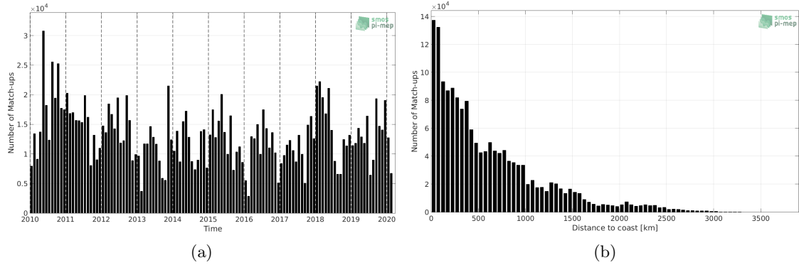
Figure 1: Number of match-ups between TSG (LEGOS-DM) and SMOS SSS L3 v7 - 9 Days (CATDS-CECOS-LOCEAN) SSS as a function of time (a) and as function of the distance to coast (b) over the Tropical Pacific Ocean Pi-MEP region and for the full satellite product period.
