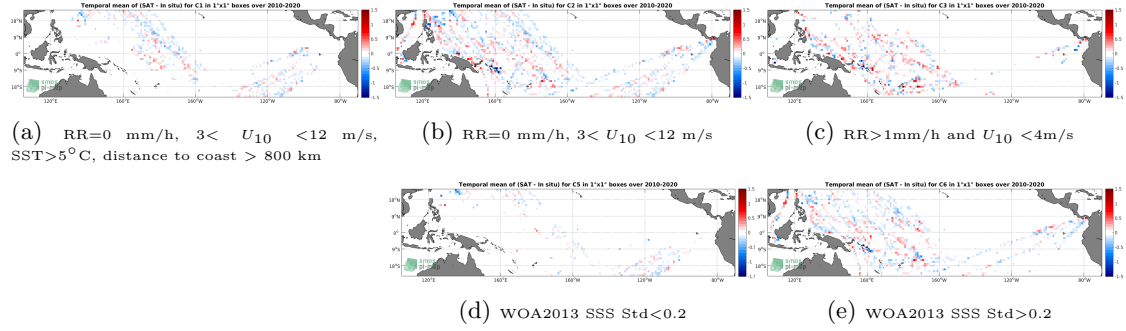
Figure 12: Temporal mean gridded over spatial boxes of size 1^{\circ}\times 1^{\circ} of \Delta\text{SSS} (SMOS SSS L3 v7 - 9 Days (CATDS-CECOS-LOCEAN) - TSG (LEGOS-DM)) for 5 different subdatasets corresponding to:RR=0 mm/h, 3 < U_{10} < 12 m/s, SST >5^{\circ}\text{C} , distance to coast > 800 km (a), RR=0 mm/h, 3 < U_{10} < 12 m/s (b), RR >1 mm/h and U_{10} < 4 m/s (c), WOA2013 SSS Std <0.2 (d), WOA2013 SSS Std >0.2 (e).
