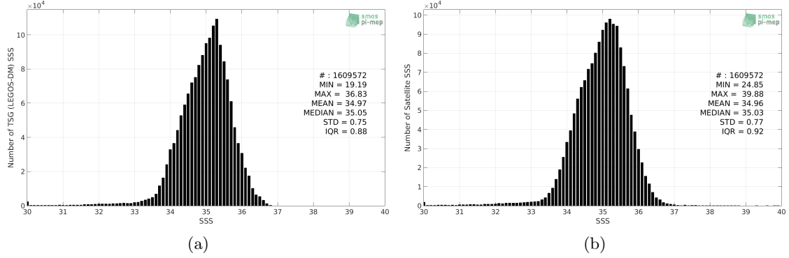
Figure 2: Histograms of SSS from TSG (LEGOS-DM) (a) and SMOS SSS L3 v7 - 9 Days (CATDS-CECOS-LOCEAN) (b) considering all match-up pairs per bins of 0.1 over the Tropical Pacific Ocean Pi-MEP region and for the full satellite product period.
