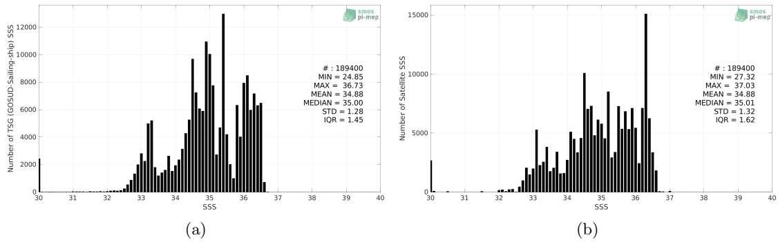
Figure 2: Histograms of SSS from TSG (GOSUD-Sailing-ship) (a) and SMOS SSS L3 v7 - 9 Days (CATDS-CECOS-LOCEAN) (b) considering all match-up pairs per bins of 0.1 over the Tropical Pacific Ocean Pi-MEP region and for the full satellite product period.
