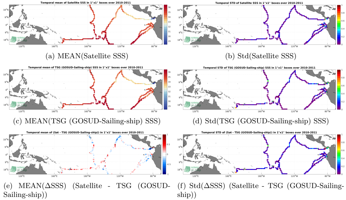
Figure 6: Temporal mean (left) and Std (right) of SSS from SMOS SSS L3 v7 - 9 Days (CATDS-CECOS-LOCEAN) (top), TSG (GOSUD-Sailing-ship) (middle), and of \Delta SSS (Satellite - TSG (GOSUD-Sailing-ship)). Only match-up pairs are used to generate these maps.
