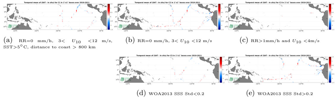
Figure 12: Temporal mean gridded over spatial boxes of size 1^{\circ}\times 1^{\circ} of \Delta SSS (SMOS SSS L3 v7 - 9 Days (CATDS-CECOS-LOCEAN) - TSG (GOSUD-Sailing-ship)) for 5 different subdatasets corresponding to:RR=0 mm/h, 3 < U_{10} < 12 m/s, SST >5^{\circ}\text{C} , distance to coast > 800 km (a), RR=0 mm/h, 3 < U_{10} < 12 m/s (b), RR >1 mm/h and U_{10} < 4 m/s (c), WOA2013 SSS Std <0.2 (d), WOA2013 SSS Std >0.2 (e).
