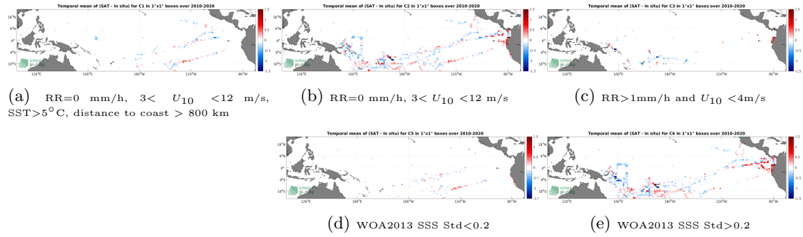
Figure 12: Temporal mean gridded over spatial boxes of size 1^{\circ}\times 1^{\circ} of \Delta SSS (SMOS SSS L3 v7 - 9 Days (CATDS-CECOS-LOCEAN) - TSG (GOSUD-Research-vessel)) for 5 different subdatasets corresponding to:RR=0 mm/h, 3 < U_{10} < 12 m/s, SST >5^{\circ}\text{C} , distance to coast > 800 km (a), RR=0 mm/h, 3 < U_{10} < 12 m/s (b), RR >1 mm/h and U_{10} < 4 m/s (c), WOA2013 SSS Std <0.2 (d), WOA2013 SSS Std >0.2 (e).
