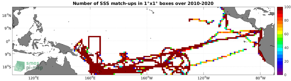
Figure 4: Number of SSS match-ups between TSG (GOSUD-Research-vessel) SSS and the SMOS SSS L3 v7 - 9 Days (CATDS-CECOS-LOCEAN) SSS product for the Tropical Pacific Ocean Pi-MEP region over 1^\circ \times 1^\circ boxes and for the full satellite product period.
