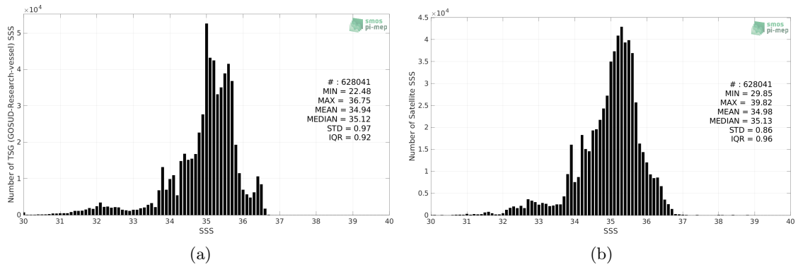
Figure 2: Histograms of SSS from TSG (GOSUD-Research-vessel) (a) and SMOS SSS L3 v7 - 9 Days (CATDS-CECOS-LOCEAN) (b) considering all match-up pairs per bins of 0.1 over the Tropical Pacific Ocean Pi-MEP region and for the full satellite product period.
