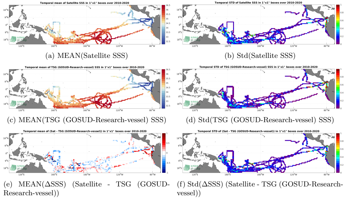
Figure 6: Temporal mean (left) and Std (right) of SSS from SMOS SSS L3 v7 - 9 Days (CATDS-CECOS-LOCEAN) (top), TSG (GOSUD-Research-vessel) (middle), and of \Delta SSS (Satellite - TSG (GOSUD-Research-vessel)). Only match-up pairs are used to generate these maps.
