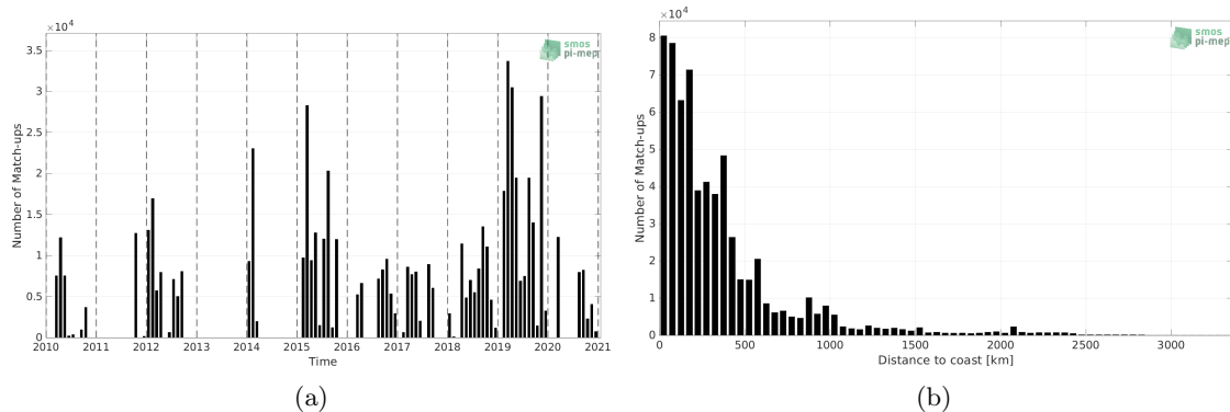
Figure 1: Number of match-ups between TSG (GOSUD-Research-vessel) and SMOS SSS L3 v7 - 9 Days (CATDS-CECOS-LOCEAN) SSS as a function of time (a) and as function of the distance to coast (b) over the Tropical Pacific Ocean Pi-MEP region and for the full satellite product period.
