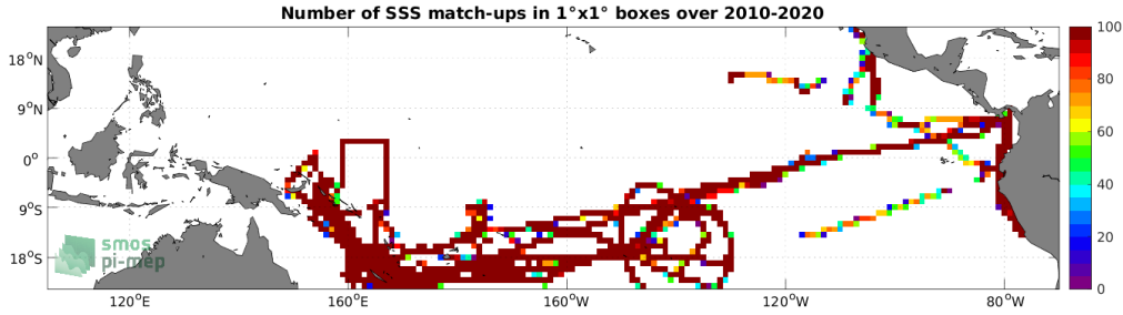
Figure 4: Number of SSS match-ups between TSG (GOSUD-Research-vessel) SSS and the SMOS SSS L3 v7 - 9 Days (CATDS-CECOS-LOCEAN) SSS product for the Tropical Pacific Ocean Pi-MEP region over 1^\circ \times 1^\circ boxes and for the full satellite product period.
