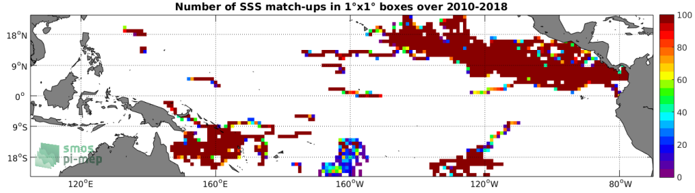
Figure 3: Number of SSS match-ups between Surface drifters SSS and the SMOS SSS L3 v7 - 9 Days (CATDS-CECOS-LOCEAN) SSS product for the Tropical Pacific Ocean Pi-MEP region over 1^\circ \times 1^\circ boxes and for the full satellite product period.
