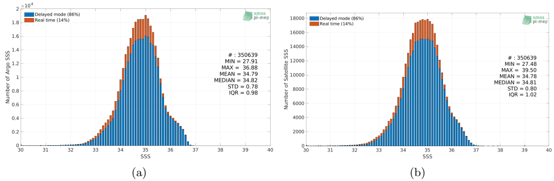
Figure 2: Histograms of SSS from Argo (a) and SMOS SSS L3 v7 - 9 Days (CATDS-CECOS-LOCEAN) (b) considering all match-up pairs per bins of 0.1 over the Tropical Pacific Ocean Pi-MEP region and for the full satellite product period.
