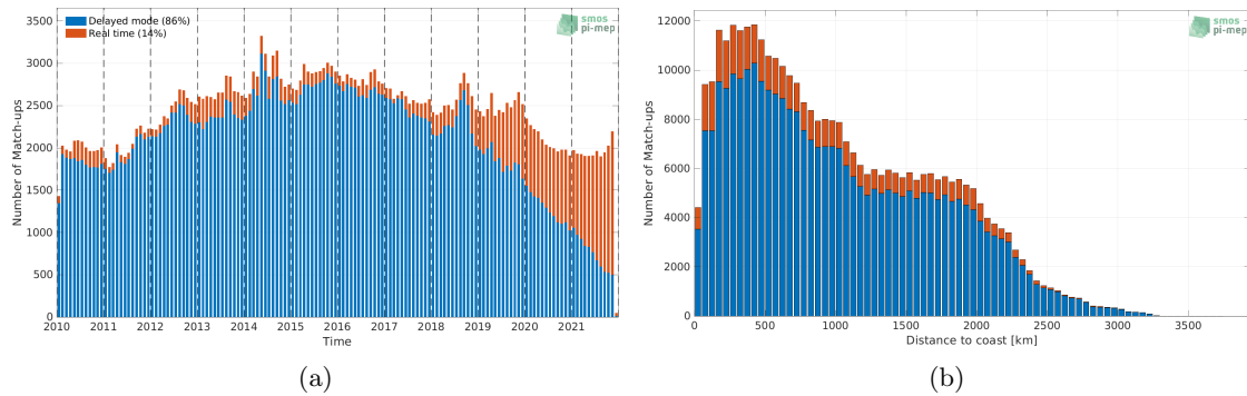
Figure 1: Number of match-ups between Argo and SMOS SSS L3 v7 - 9 Days (CATDS-CECOS-LOCEAN) SSS as a function of time (a) and as function of the distance to coast (b) over the Tropical Pacific Ocean Pi-MEP region and for the full satellite product period.
