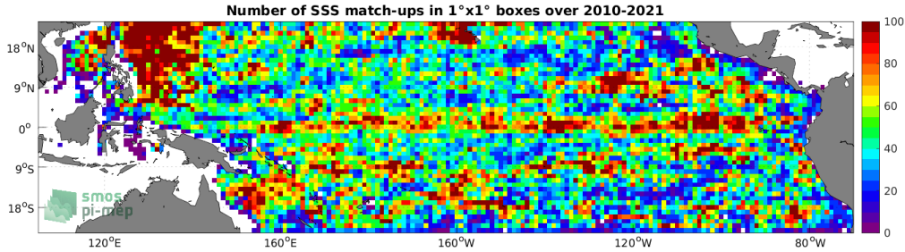
Figure 4: Number of SSS match-ups between Argo SSS and the SMOS SSS L3 v7 - 9 Days (CATDS-CECOS-LOCEAN) SSS product for the Tropical Pacific Ocean Pi-MEP region over 1^\circ \times 1^\circ boxes and for the full satellite product period.
