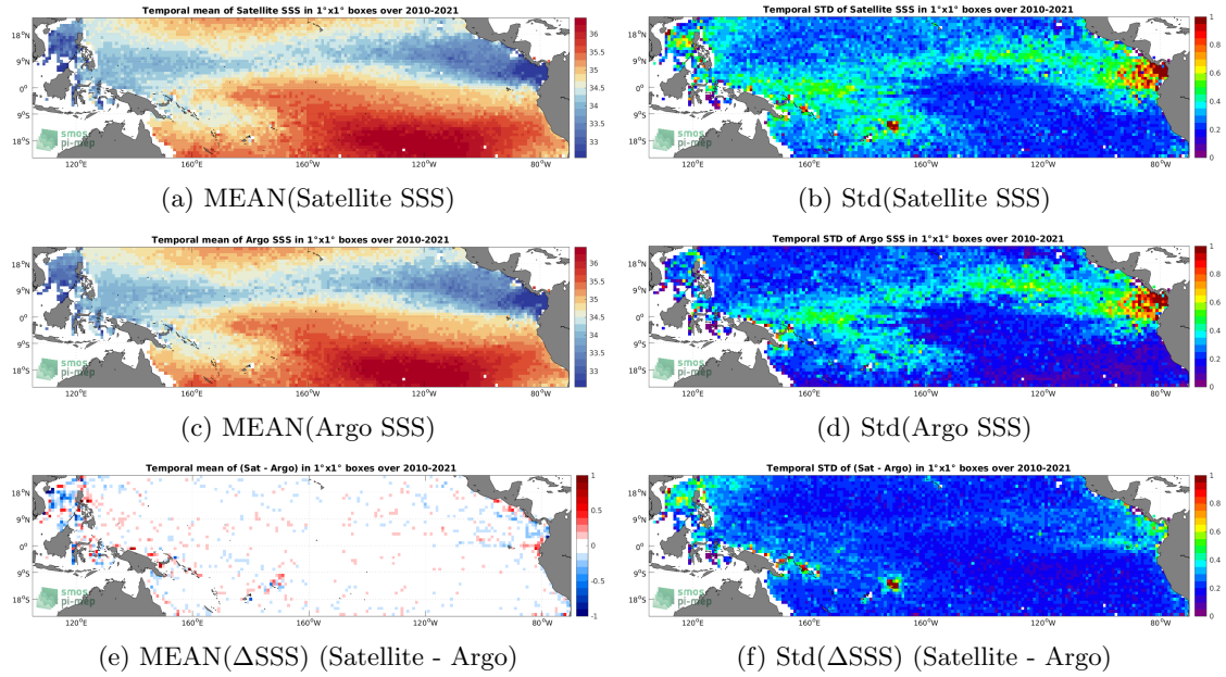
Figure 6: Temporal mean (left) and Std (right) of SSS from SMOS SSS L3 v7 - 9 Days (CATDS-CECOS-LOCEAN) (top), Argo (middle), and of \Delta SSS (Satellite - Argo). Only match-up pairs are used to generate these maps.
