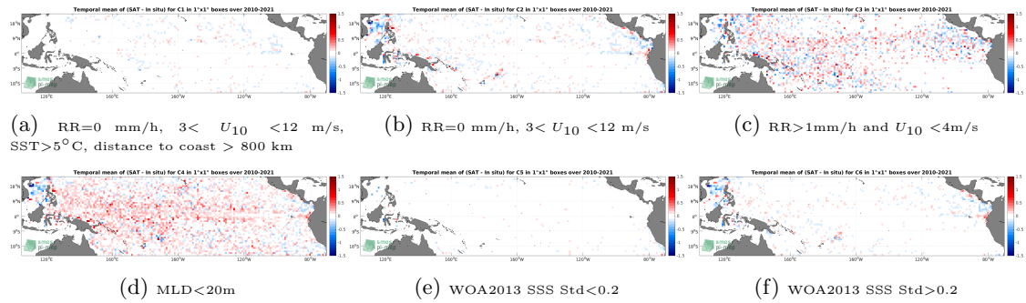
Figure 12: Temporal mean gridded over spatial boxes of size 1^\circ \times 1^\circ of \Delta SSS (SMOS SSS L3 v7 - 9 Days (CATDS-CECOS-LOCEAN) - Argo) for 6 different subdatasets corresponding to:RR=0 mm/h, 3 < U_{10} < 12 m/s, SST >5^\circ C, distance to coast > 800 km (a), RR=0 mm/h, 3 < U_{10} < 12 m/s (b), RR >1 mm/h and U_{10} < 4 m/s (c),MLD <20 m (d),WOA2013 SSS Std <0.2 (e),WOA2013 SSS Std >0.2 (f).
