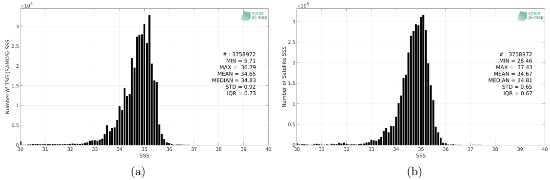
Figure 2: Histograms of SSS from TSG (SAMOS) (a) and SMOS SSS L3 v7 - 18 Days (CATDS-CECOS-LOCEAN) (b) considering all match-up pairs per bins of 0.1 over the Tropical Pacific Ocean Pi-MEP region and for the full satellite product period.
