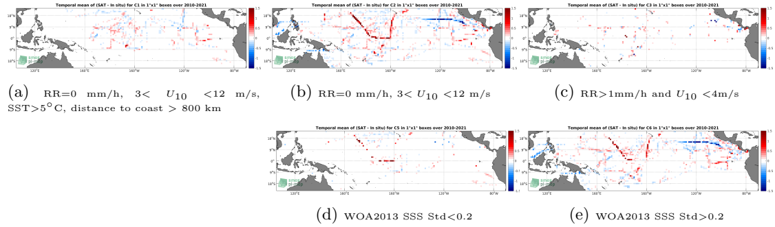
Figure 12: Temporal mean gridded over spatial boxes of size 1^{\circ}\times 1^{\circ} of \Delta\text{SSS} (SMOS SSS L3 v7 - 18 Days (CATDS-CECOS-LOCEAN) - TSG (SAMOS)) for 5 different subdatasets corresponding to:RR=0 mm/h, 3 < U_{10} < 12 m/s, SST >5^{\circ}\text{C} , distance to coast > 800 km (a), RR=0 mm/h, 3 < U_{10} < 12 m/s (b), RR >1 mm/h and U_{10} < 4 m/s (c), WOA2013 SSS Std <0.2 (d), WOA2013 SSS Std >0.2 (e).
