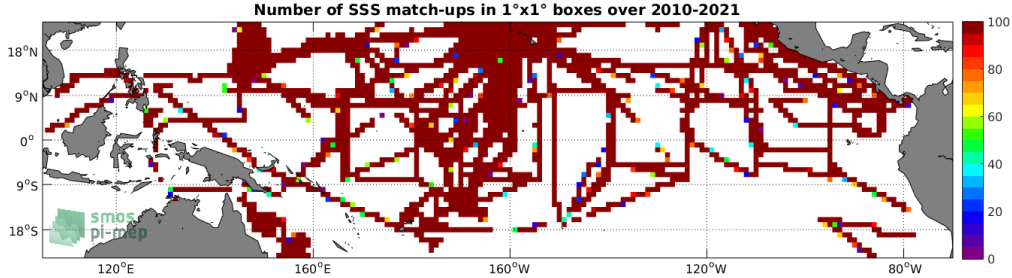
Figure 4: Number of SSS match-ups between TSG (SAMOS) SSS and the SMOS SSS L3 v7 - 18 Days (CATDS-CECOS-LOCEAN) SSS product for the Tropical Pacific Ocean Pi-MEP region over 1^\circ \times 1^\circ boxes and for the full satellite product period.
