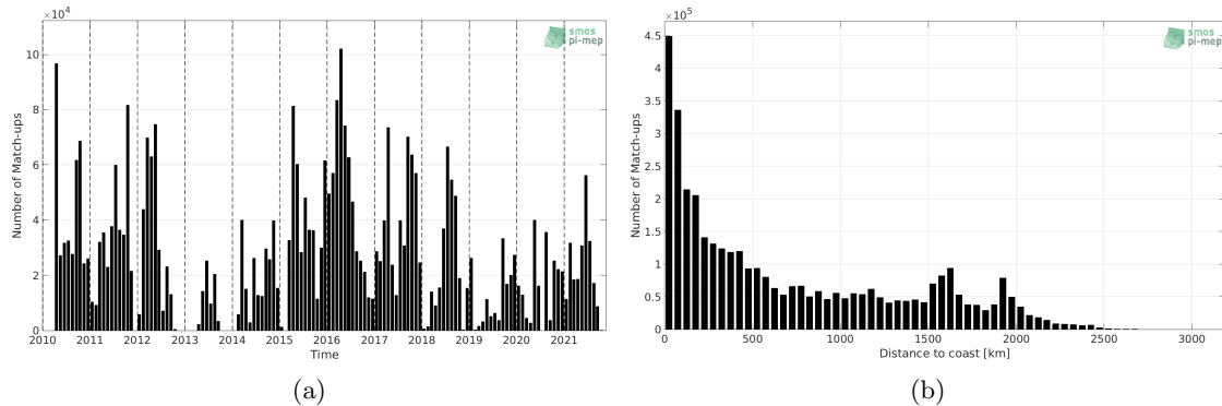
Figure 1: Number of match-ups between TSG (SAMOS) and SMOS SSS L3 v7 - 18 Days (CATDS-CECOS-LOCEAN) SSS as a function of time (a) and as function of the distance to coast (b) over the Tropical Pacific Ocean Pi-MEP region and for the full satellite product period.
