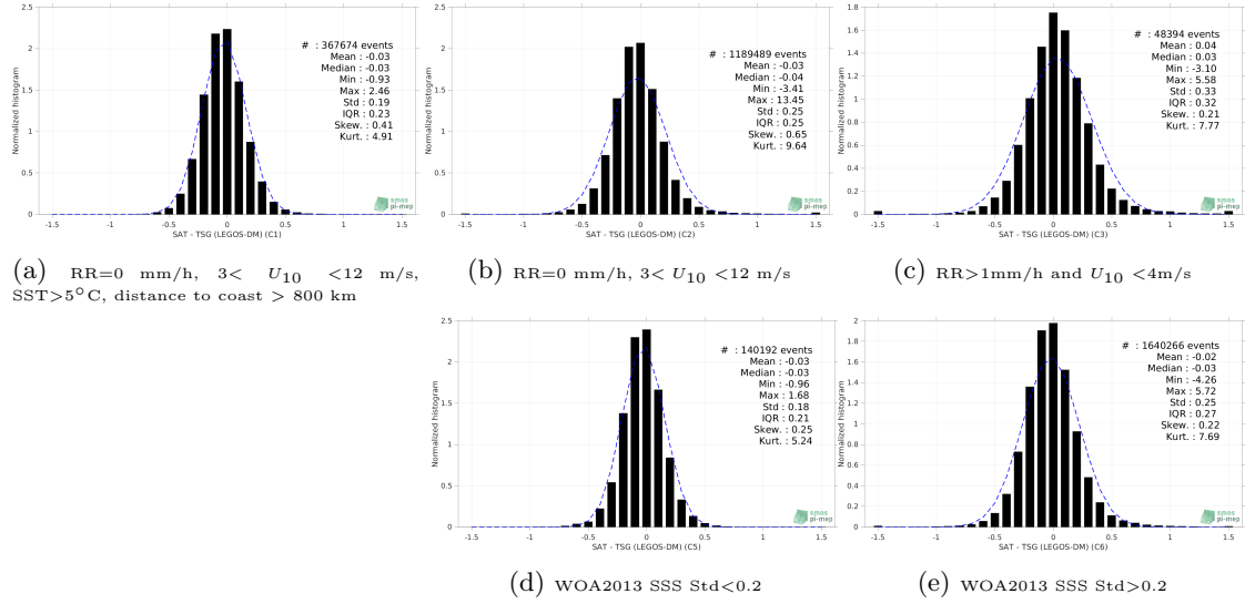
Figure 13: Normalized histogram of \Delta\text{SSS} (SMOS SSS L3 v7 - 18 Days (CATDS-CECOS-LOCEAN) - TSG (LEGOS-DM)) for 5 different subdatasets corresponding to: RR=0 mm/h, 3 < U_{10} < 12 m/s, SST>5°C, distance to coast > 800 km (a), RR=0 mm/h, 3 < U_{10} < 12 m/s (b), RR>1mm/h and U_{10} < 4 m/s (c), WOA2013 SSS Std<0.2 (d), WOA2013 SSS Std>0.2 (e).
