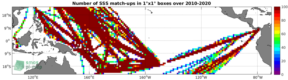
Figure 4: Number of SSS match-ups between TSG (LEGOS-DM) SSS and the SMOS SSS L3 v7 - 18 Days (CATDS-CECOS-LOCEAN) SSS product for the Tropical Pacific Ocean Pi-MEP region over 1^\circ \times 1^\circ boxes and for the full satellite product period.
