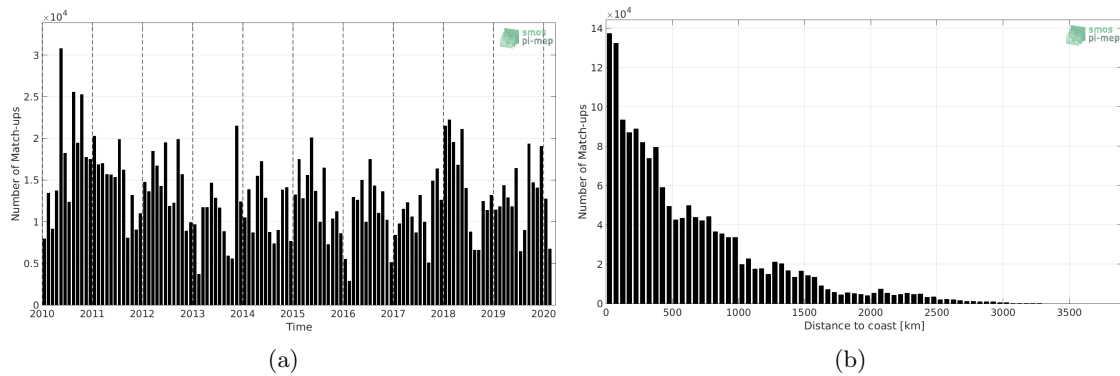
Figure 1: Number of match-ups between TSG (LEGOS-DM) and SMOS SSS L3 v7 - 18 Days (CATDS-CECOS-LOCEAN) SSS as a function of time (a) and as function of the distance to coast (b) over the Tropical Pacific Ocean Pi-MEP region and for the full satellite product period.
