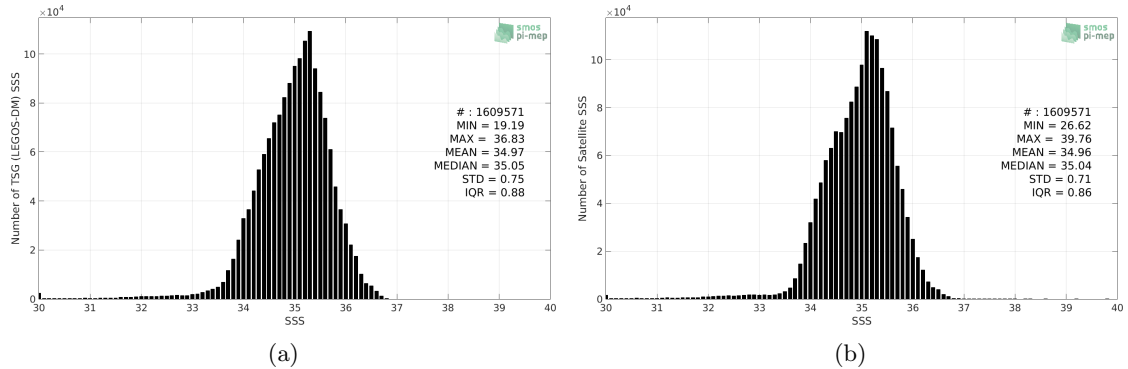
Figure 2: Histograms of SSS from TSG (LEGOS-DM) (a) and SMOS SSS L3 v7 - 18 Days (CATDS-CECOS-LOCEAN) (b) considering all match-up pairs per bins of 0.1 over the Tropical Pacific Ocean Pi-MEP region and for the full satellite product period.
