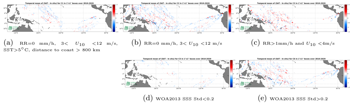
Figure 12: Temporal mean gridded over spatial boxes of size 1^{\circ}\times 1^{\circ} of \Delta\text{SSS} (SMOS SSS L3 v7 - 18 Days (CATDS-CECOS-LOCEAN) - TSG (LEGOS-DM)) for 5 different subdatasets corresponding to:RR=0 mm/h, 3 < U_{10} < 12 m/s, SST > 5^{\circ}\text{C} , distance to coast > 800 km (a), RR=0 mm/h, 3 < U_{10} < 12 m/s (b), RR > 1 mm/h and U_{10} < 4 m/s (c), WOA2013 SSS Std < 0.2 (d), WOA2013 SSS Std > 0.2 (e).
