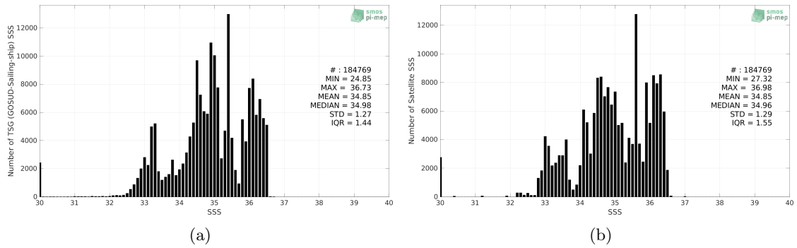
Figure 2: Histograms of SSS from TSG (GOSUD-Sailing-ship) (a) and SMOS SSS L3 v7 - 18 Days (CATDS-CECOS-LOCEAN) (b) considering all match-up pairs per bins of 0.1 over the Tropical Pacific Ocean Pi-MEP region and for the full satellite product period.
