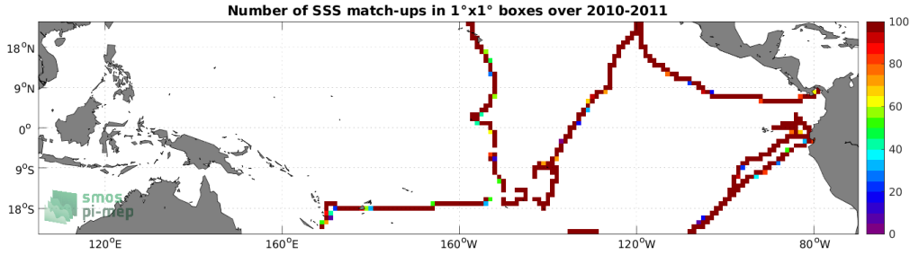
Figure 4: Number of SSS match-ups between TSG (GOSUD-Sailing-ship) SSS and the SMOS SSS L3 v7 - 18 Days (CATDS-CECOS-LOCEAN) SSS product for the Tropical Pacific Ocean Pi-MEP region over 1^\circ \times 1^\circ boxes and for the full satellite product period.
