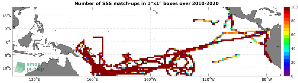
Figure 4: Number of SSS match-ups between TSG (GOSUD-Research-vessel) SSS and the SMOS SSS L3 v7 - 18 Days (CATDS-CECOS-LOCEAN) SSS product for the Tropical Pacific Ocean Pi-MEP region over 1^\circ \times 1^\circ boxes and for the full satellite product period.
