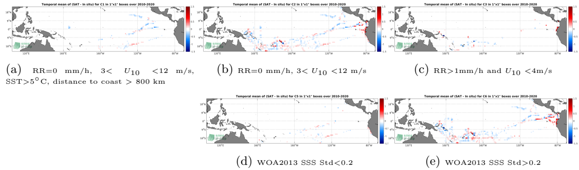
Figure 12: Temporal mean gridded over spatial boxes of size 1^\circ \times 1^\circ of \Delta SSS (SMOS SSS L3 v7 - 18 Days (CATDS-CECOS-LOCEAN) - TSG (GOSUD-Research-vessel)) for 5 different sub-datasets corresponding to: RR=0 mm/h, 3 < U_{10} < 12 m/s, SST > 5^\circ\text{C} , distance to coast > 800 km (a), RR=0 mm/h, 3 < U_{10} < 12 m/s (b), RR > 1 mm/h and U_{10} < 4 m/s (c), WOA2013 SSS Std < 0.2 (d), WOA2013 SSS Std > 0.2 (e).
