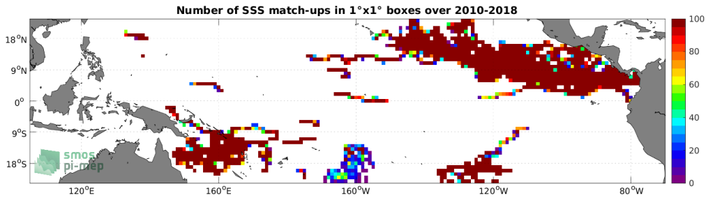
Figure 3: Number of SSS match-ups between Surface drifters SSS and the SMOS SSS L3 v7 - 18 Days (CATDS-CECOS-LOCEAN) SSS product for the Tropical Pacific Ocean Pi-MEP region over 1^\circ \times 1^\circ boxes and for the full satellite product period.
