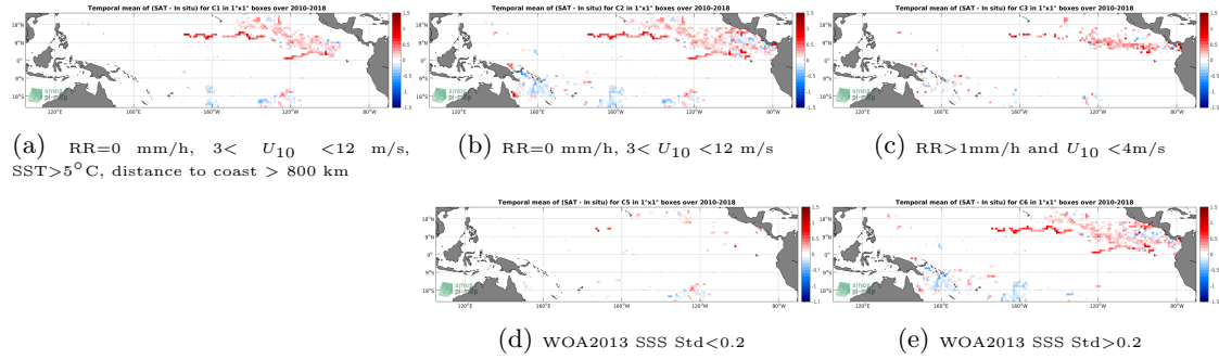
Figure 11: Temporal mean gridded over spatial boxes of size 1^{\circ}\times 1^{\circ} of \Delta\text{SSS} (SMOS SSS L3 v7 - 18 Days (CATDS-CECOS-LOCEAN) - Surface drifters) for 5 different subdatasets corresponding to:RR=0 mm/h, 3 < U_{10} < 12 m/s, SST >5^{\circ}\text{C} , distance to coast > 800 km (a), RR=0 mm/h, 3 < U_{10} < 12 m/s (b), RR >1 mm/h and U_{10} < 4 m/s (c), WOA2013 SSS Std <0.2 (d), WOA2013 SSS Std >0.2 (e).
