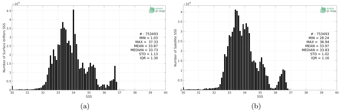
Figure 2: Histograms of SSS from Surface drifters (a) and SMOS SSS L3 v7 - 18 Days (CATDS-CECOS-LOCEAN) (b) considering all match-up pairs per bins of 0.1 over the Tropical Pacific Ocean Pi-MEP region and for the full satellite product period.
