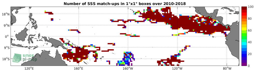
Figure 3: Number of SSS match-ups between Surface drifters SSS and the SMOS SSS L3 v7 - 18 Days (CATDS-CECOS-LOCEAN) SSS product for the Tropical Pacific Ocean Pi-MEP region over 1^\circ \times 1^\circ boxes and for the full satellite product period.
