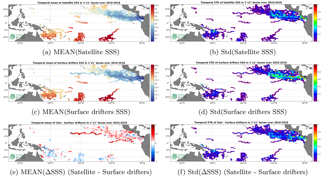
Figure 5: Temporal mean (left) and Std (right) of SSS from SMOS SSS L3 v7 - 18 Days (CATDS-CECOS-LOCEAN) (top), Surface drifters (middle), and of \Delta SSS (Satellite - Surface drifters). Only match-up pairs are used to generate these maps.
