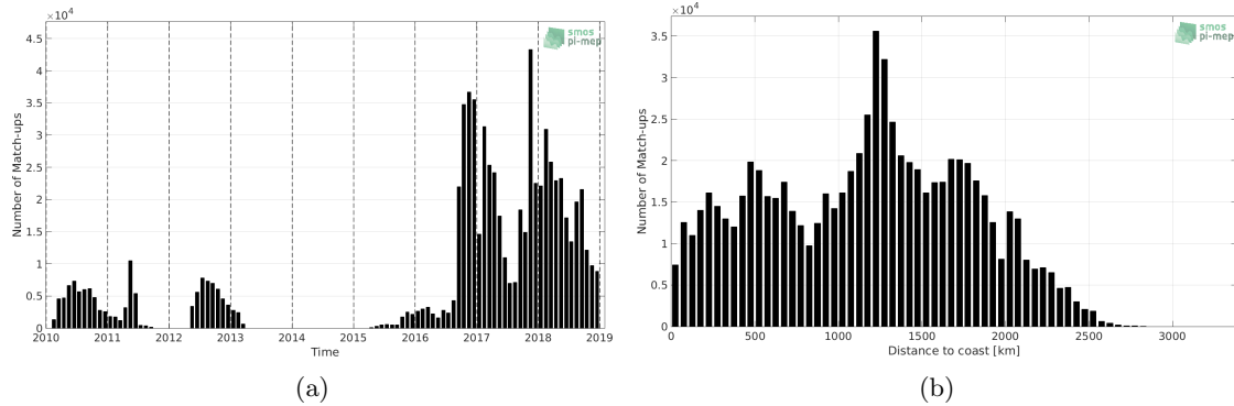
Figure 1: Number of match-ups between Surface drifters and SMOS SSS L3 v7 - 18 Days (CATDS-CECOS-LOCEAN) SSS as a function of time (a) and as function of the distance to coast (b) over the Tropical Pacific Ocean Pi-MEP region and for the full satellite product period.
