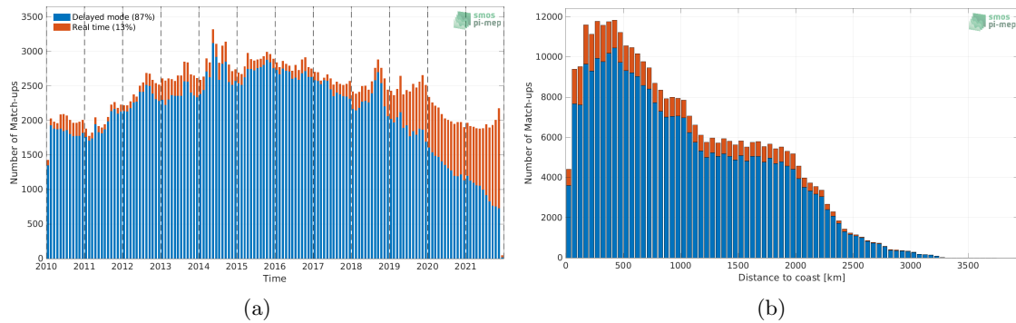
Figure 1: Number of match-ups between Argo and SMOS SSS L3 v7 - 18 Days (CATDS-CECOS-LOCEAN) SSS as a function of time (a) and as function of the distance to coast (b) over the Tropical Pacific Ocean Pi-MEP region and for the full satellite product period.
