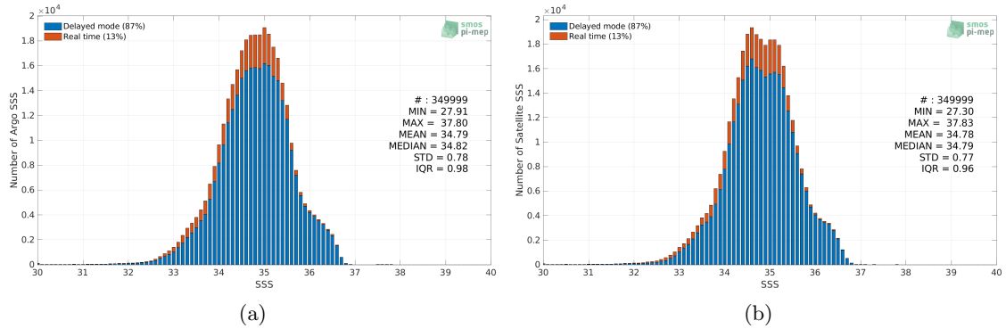
Figure 2: Histograms of SSS from Argo (a) and SMOS SSS L3 v7 - 18 Days (CATDS-CECOS-LOCEAN) (b) considering all match-up pairs per bins of 0.1 over the Tropical Pacific Ocean Pi-MEP region and for the full satellite product period.
