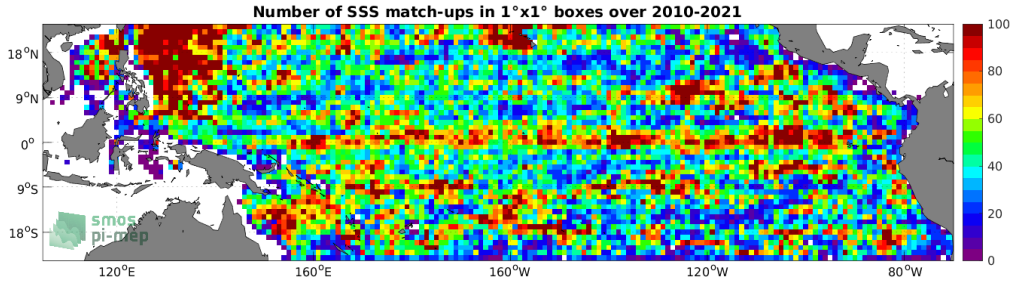
Figure 4: Number of SSS match-ups between Argo SSS and the SMOS SSS L3 v7 - 18 Days (CATDS-CECOS-LOCEAN) SSS product for the Tropical Pacific Ocean Pi-MEP region over 1^\circ \times 1^\circ boxes and for the full satellite product period.
