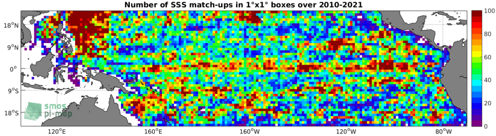
Figure 4: Number of SSS match-ups between Argo SSS and the SMOS SSS L3 v7 - 18 Days (CATDS-CECOS-LOCEAN) SSS product for the Tropical Pacific Ocean Pi-MEP region over 1^\circ \times 1^\circ boxes and for the full satellite product period.
