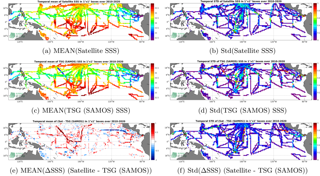
Figure 6: Temporal mean (left) and Std (right) of SSS from SMOS SSS L3 v5 - 9 Days (CATDS-CECOS-LOCEAN) (top), TSG (SAMOS) (middle), and of \Delta SSS (Satellite - TSG (SAMOS)). Only match-up pairs are used to generate these maps.
