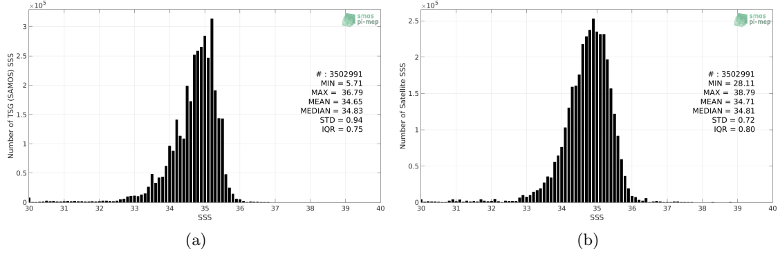
Figure 2: Histograms of SSS from TSG (SAMOS) (a) and SMOS SSS L3 v5 - 9 Days (CATDS-CECOS-LOCEAN) (b) considering all match-up pairs per bins of 0.1 over the Tropical Pacific Ocean Pi-MEP region and for the full satellite product period.
