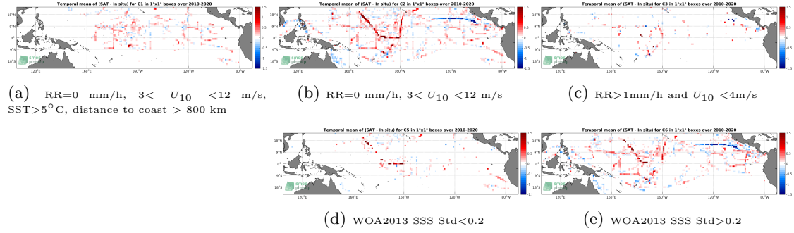
Figure 12: Temporal mean gridded over spatial boxes of size 1^{\circ} \times 1^{\circ} of \Delta\text{SSS} (SMOS SSS L3 v5 - 9 Days (CATDS-CECOS-LOCEAN) - TSG (SAMOS)) for 5 different subdatasets corresponding to:RR=0 mm/h, 3 < U_{10} < 12 m/s, SST >5^{\circ}\text{C} , distance to coast > 800 km (a), RR=0 mm/h, 3 < U_{10} < 12 m/s (b), RR >1 mm/h and U_{10} < 4 m/s (c), WOA2013 SSS Std <0.2 (d), WOA2013 SSS Std >0.2 (e).
