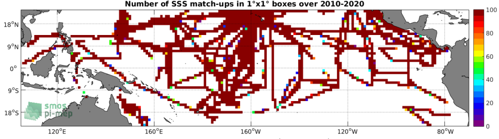
Figure 4: Number of SSS match-ups between TSG (SAMOS) SSS and the SMOS SSS L3 v5 - 9 Days (CATDS-CECOS-LOCEAN) SSS product for the Tropical Pacific Ocean Pi-MEP region over 1^\circ \times 1^\circ boxes and for the full satellite product period.
