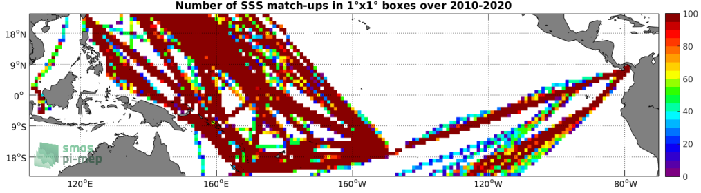
Figure 4: Number of SSS match-ups between TSG (LEGOS-DM) SSS and the SMOS SSS L3 v5 - 9 Days (CATDS-CECOS-LOCEAN) SSS product for the Tropical Pacific Ocean Pi-MEP region over 1^\circ \times 1^\circ boxes and for the full satellite product period.
