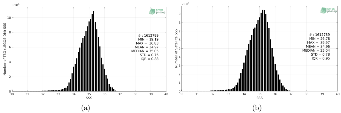
Figure 2: Histograms of SSS from TSG (LEGOS-DM) (a) and SMOS SSS L3 v5 - 9 Days (CATDS-CECOS-LOCEAN) (b) considering all match-up pairs per bins of 0.1 over the Tropical Pacific Ocean Pi-MEP region and for the full satellite product period.
