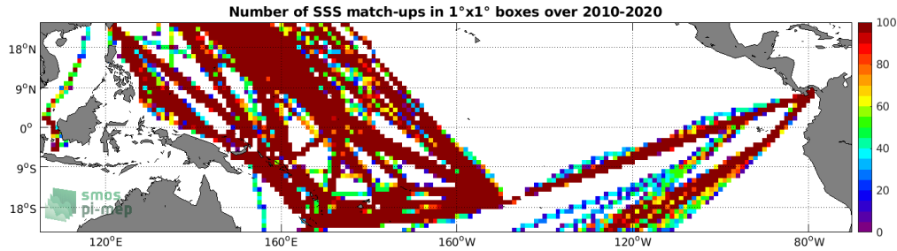
Figure 4: Number of SSS match-ups between TSG (LEGOS-DM) SSS and the SMOS SSS L3 v5 - 9 Days (CATDS-CECOS-LOCEAN) SSS product for the Tropical Pacific Ocean Pi-MEP region over 1^\circ \times 1^\circ boxes and for the full satellite product period.
