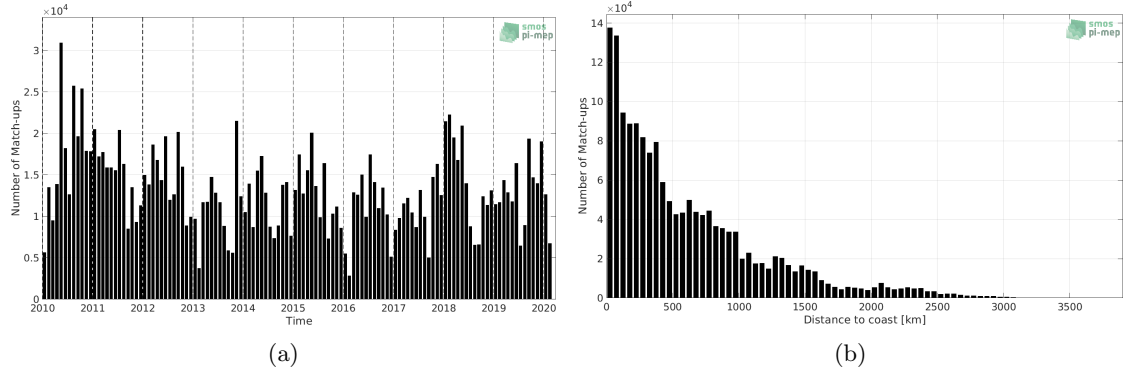
Figure 1: Number of match-ups between TSG (LEGOS-DM) and SMOS SSS L3 v5 - 9 Days (CATDS-CECOS-LOCEAN) SSS as a function of time (a) and as function of the distance to coast (b) over the Tropical Pacific Ocean Pi-MEP region and for the full satellite product period.
