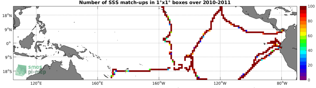
Figure 4: Number of SSS match-ups between TSG (GOSUD-Sailing-ship) SSS and the SMOS SSS L3 v5 - 9 Days (CATDS-CECOS-LOCEAN) SSS product for the Tropical Pacific Ocean Pi-MEP region over 1^\circ \times 1^\circ boxes and for the full satellite product period.
