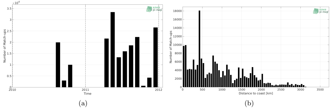
Figure 1: Number of match-ups between TSG (GOSUD-Sailing-ship) and SMOS SSS L3 v5 - 9 Days (CATDS-CECOS-LOCEAN) SSS as a function of time (a) and as function of the distance to coast (b) over the Tropical Pacific Ocean Pi-MEP region and for the full satellite product period.
