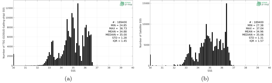
Figure 2: Histograms of SSS from TSG (GOSUD-Sailing-ship) (a) and SMOS SSS L3 v5 - 9 Days (CATDS-CECOS-LOCEAN) (b) considering all match-up pairs per bins of 0.1 over the Tropical Pacific Ocean Pi-MEP region and for the full satellite product period.
