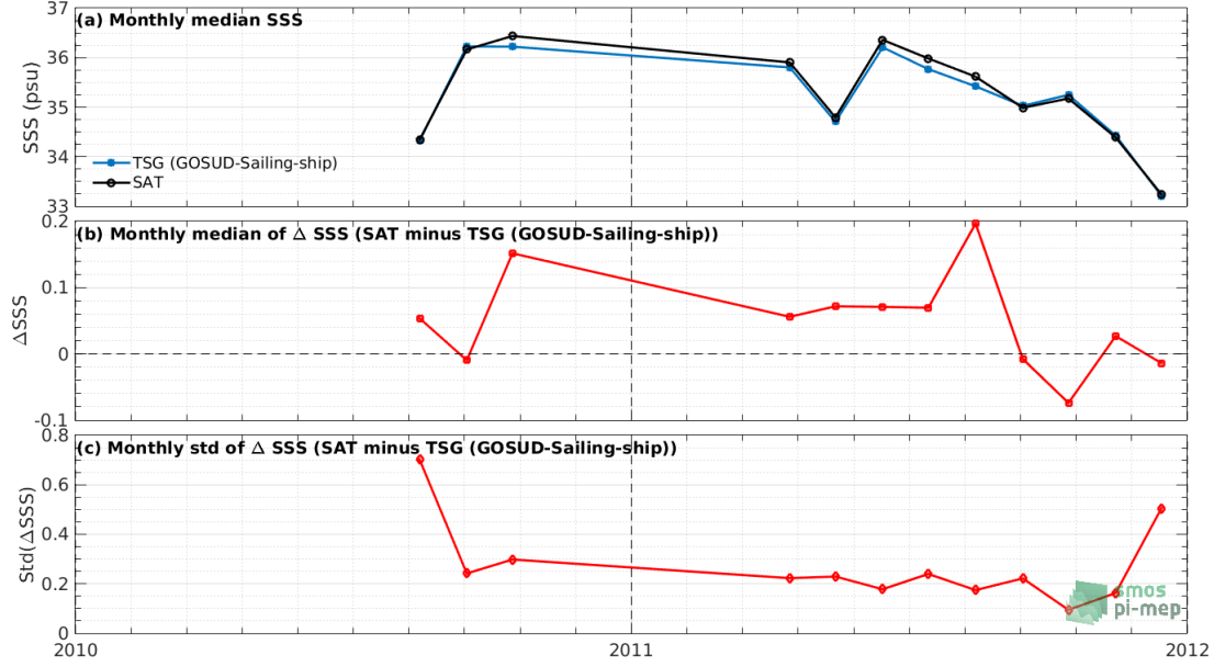
Figure 7: Time series of the monthly median SSS (top), median of \Delta\text{SSS} (Satellite - TSG (GOSUD-Sailing-ship)) and Std of \Delta\text{SSS} (Satellite - TSG (GOSUD-Sailing-ship)) over the Tropical Pacific Ocean Pi-MEP region considering all match-ups collected by the Pi-MEP.
