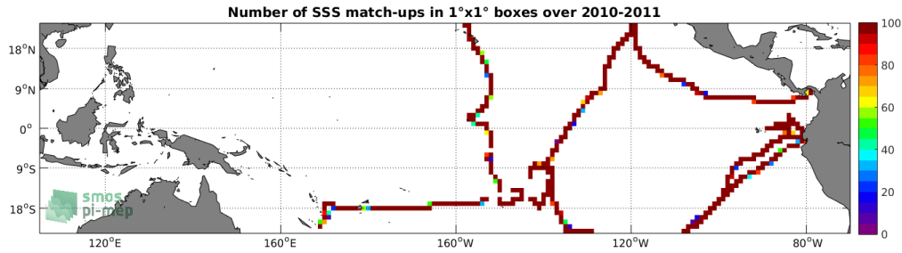
Figure 4: Number of SSS match-ups between TSG (GOSUD-Sailing-ship) SSS and the SMOS SSS L3 v5 - 9 Days (CATDS-CECOS-LOCEAN) SSS product for the Tropical Pacific Ocean Pi-MEP region over 1^\circ \times 1^\circ boxes and for the full satellite product period.
