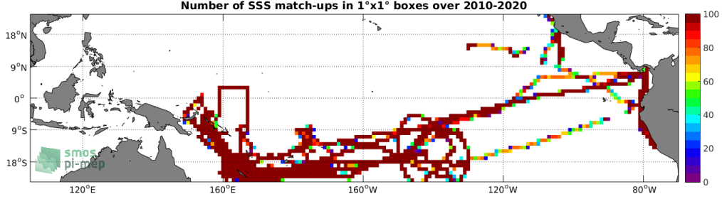
Figure 4: Number of SSS match-ups between TSG (GOSUD-Research-vessel) SSS and the SMOS SSS L3 v5 - 9 Days (CATDS-CECOS-LOCEAN) SSS product for the Tropical Pacific Ocean Pi-MEP region over 1^\circ \times 1^\circ boxes and for the full satellite product period.
