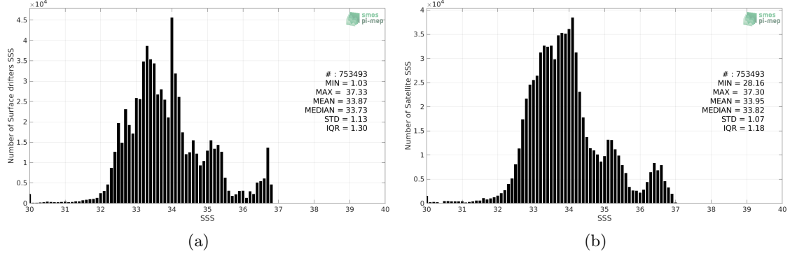
Figure 2: Histograms of SSS from Surface drifters (a) and SMOS SSS L3 v5 - 9 Days (CATDS-CECOS-LOCEAN) (b) considering all match-up pairs per bins of 0.1 over the Tropical Pacific Ocean Pi-MEP region and for the full satellite product period.
