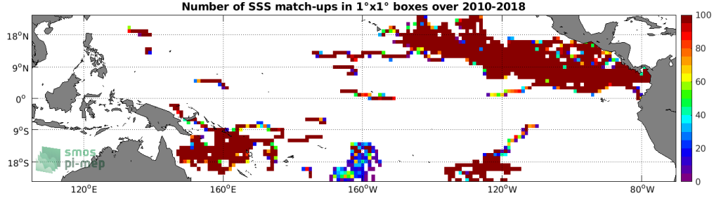
Figure 3: Number of SSS match-ups between Surface drifters SSS and the SMOS SSS L3 v5 - 9 Days (CATDS-CECOS-LOCEAN) SSS product for the Tropical Pacific Ocean Pi-MEP region over 1^\circ \times 1^\circ boxes and for the full satellite product period.
