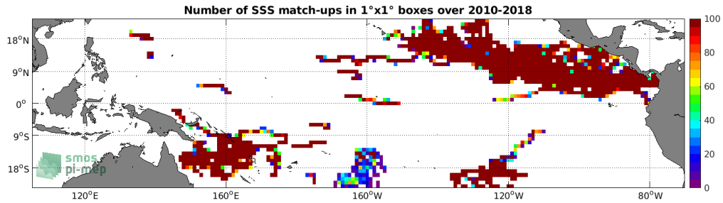
Figure 3: Number of SSS match-ups between Surface drifters SSS and the SMOS SSS L3 v5 - 9 Days (CATDS-CECOS-LOCEAN) SSS product for the Tropical Pacific Ocean Pi-MEP region over 1^\circ \times 1^\circ boxes and for the full satellite product period.
