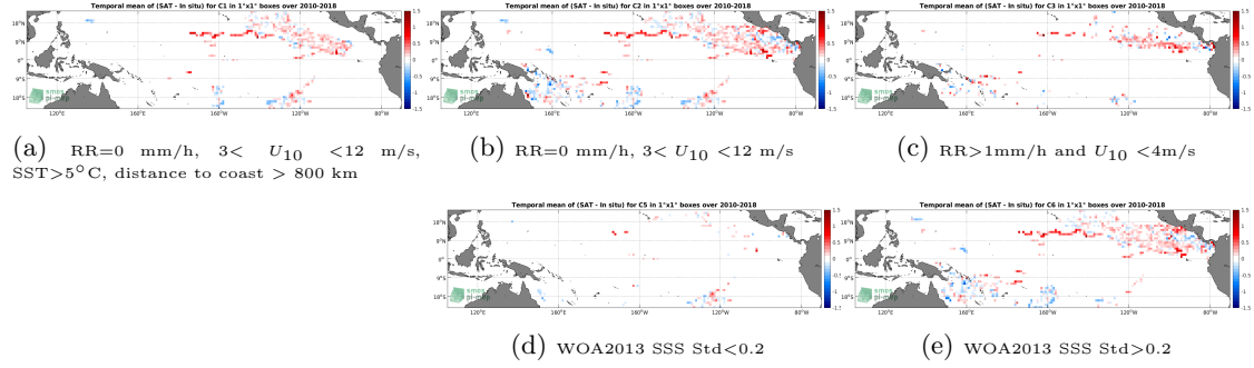
Figure 11: Temporal mean gridded over spatial boxes of size 1^{\circ}\times 1^{\circ} of \Delta\text{SSS} (SMOS SSS L3 v5 - 9 Days (CATDS-CECOS-LOCEAN) - Surface drifters) for 5 different subdatasets corresponding to: \text{RR}=0 mm/h, 3 < U_{10} < 12 m/s, \text{SST}>5^{\circ}\text{C} , distance to coast > 800 km (a), \text{RR}=0 mm/h, 3 < U_{10} < 12 m/s (b), \text{RR}>1\text{mm/h} and U_{10} < 4\text{m/s} (c), WOA2013 SSS Std <0.2 (d), WOA2013 SSS Std >0.2 (e).
