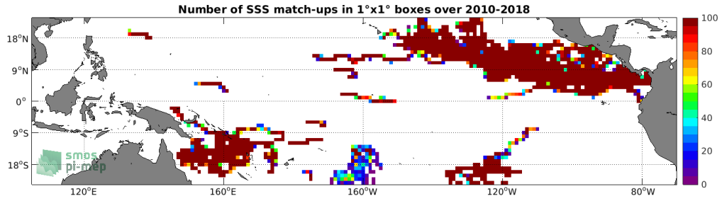
Figure 3: Number of SSS match-ups between Surface drifters SSS and the SMOS SSS L3 v5 - 9 Days (CATDS-CECOS-LOCEAN) SSS product for the Tropical Pacific Ocean Pi-MEP region over 1°x1° boxes and for the full satellite product period.
