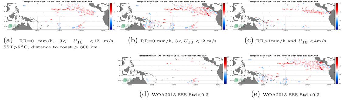
Figure 11: Temporal mean gridded over spatial boxes of size 1^{\circ}\times 1^{\circ} of \Delta\text{SSS} (SMOS SSS L3 v5 - 9 Days (CATDS-CECOS-LOCEAN) - Surface drifters) for 5 different subdatasets corresponding to:RR=0 mm/h, 3 < U_{10} < 12 m/s, SST >5^{\circ}\text{C} , distance to coast > 800 km (a), RR=0 mm/h, 3 < U_{10} < 12 m/s (b), RR >1 mm/h and U_{10} < 4 m/s (c), WOA2013 SSS Std <0.2 (d), WOA2013 SSS Std >0.2 (e).
