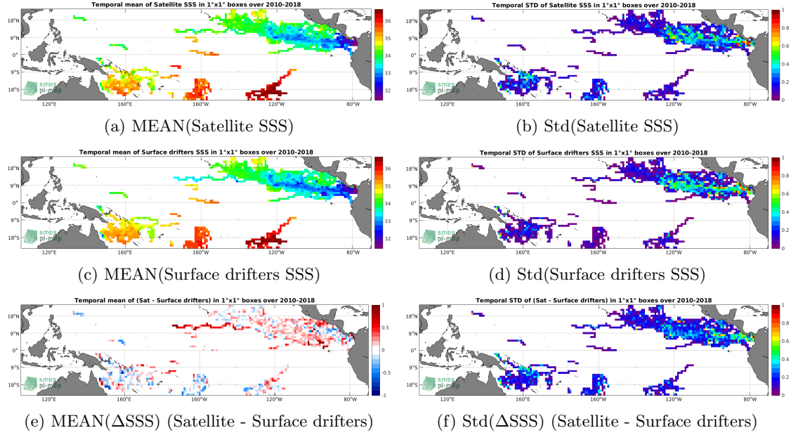
Figure 5: Temporal mean (left) and Std (right) of SSS from SMOS SSS L3 v5 - 9 Days (CATDS-CECOS-LOCEAN) (top), Surface drifters (middle), and of \Delta SSS (Satellite - Surface drifters). Only match-up pairs are used to generate these maps.
