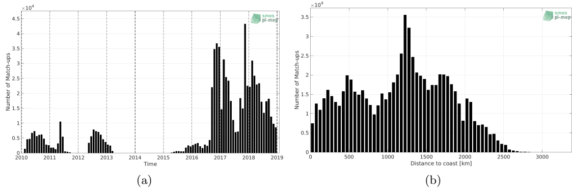
Figure 1: Number of match-ups between Surface drifters and SMOS SSS L3 v5 - 9 Days (CATDS-CECOS-LOCEAN) SSS as a function of time (a) and as function of the distance to coast (b) over the Tropical Pacific Ocean Pi-MEP region and for the full satellite product period.
