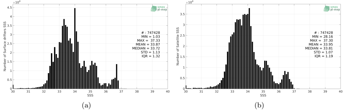
Figure 2: Histograms of SSS from Surface drifters (a) and SMOS SSS L3 v5 - 9 Days (CATDS-CECOS-LOCEAN) (b) considering all match-up pairs per bins of 0.1 over the Tropical Pacific Ocean Pi-MEP region and for the full satellite product period.
