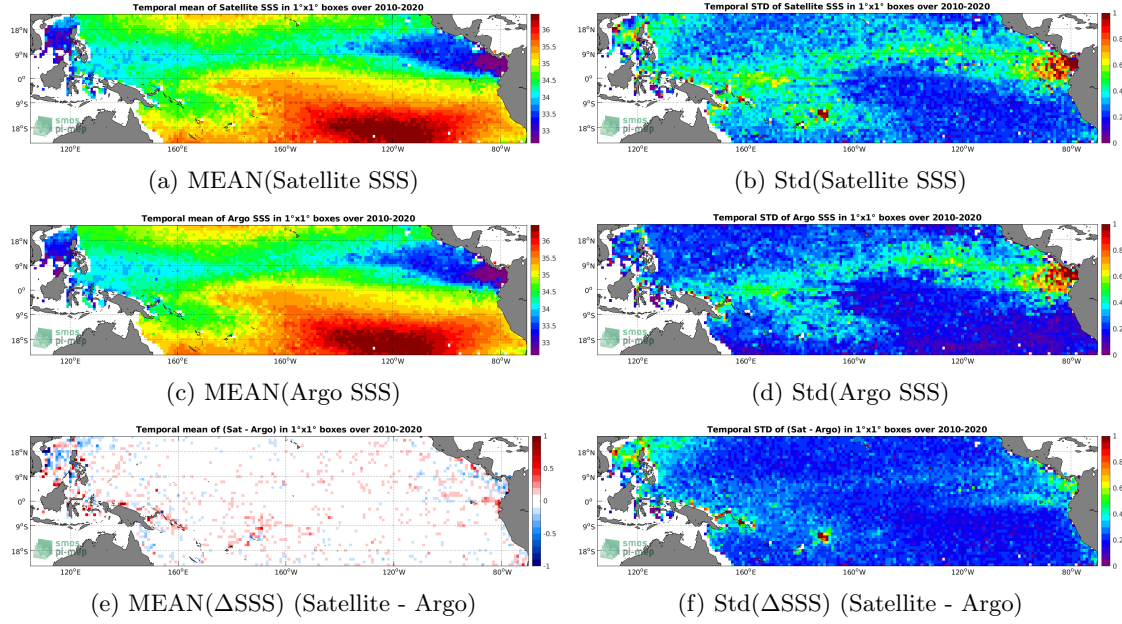
Figure 6: Temporal mean (left) and Std (right) of SSS from SMOS SSS L3 v5 - 9 Days (CATDS-CECOS-LOCEAN) (top), Argo (middle), and of \Delta SSS (Satellite - Argo). Only match-up pairs are used to generate these maps.
