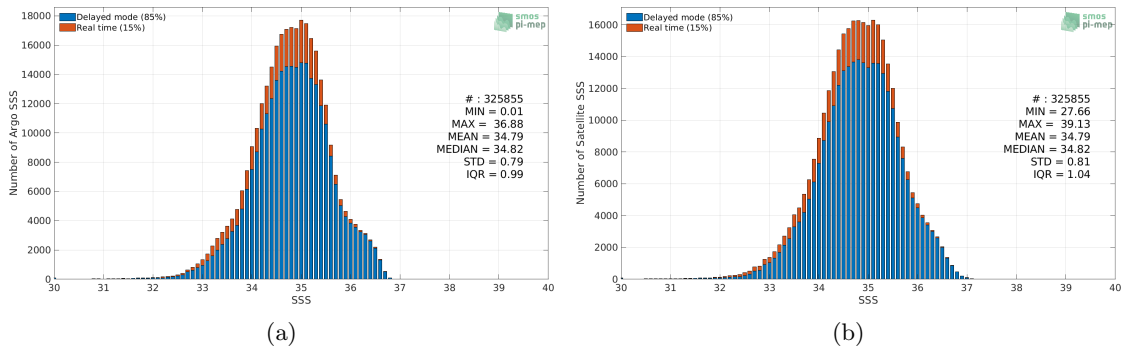
Figure 2: Histograms of SSS from Argo (a) and SMOS SSS L3 v5 - 9 Days (CATDS-CECOS-LOCEAN) (b) considering all match-up pairs per bins of 0.1 over the Tropical Pacific Ocean Pi-MEP region and for the full satellite product period.
