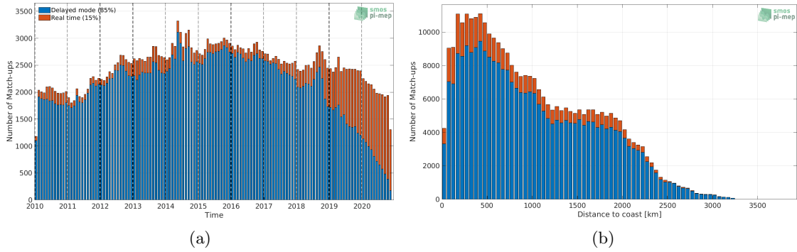
Figure 1: Number of match-ups between Argo and SMOS SSS L3 v5 - 9 Days (CATDS-CECOS-LOCEAN) SSS as a function of time (a) and as function of the distance to coast (b) over the Tropical Pacific Ocean Pi-MEP region and for the full satellite product period.
