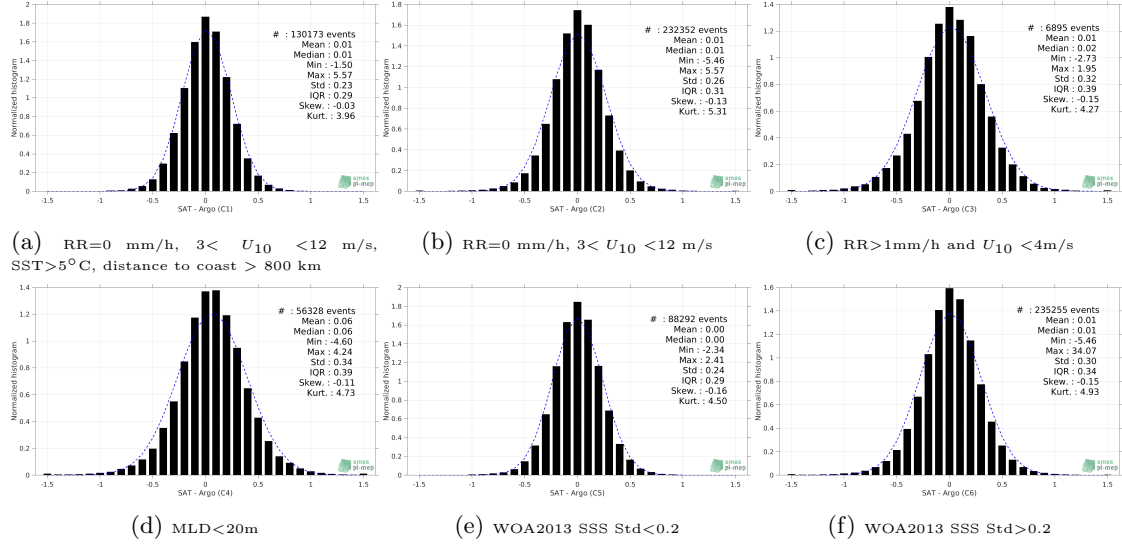
Figure 13: Normalized histogram of \Delta\text{SSS} (SMOS SSS L3 v5 - 9 Days (CATDS-CECOS-LOCEAN) - Argo) for 6 different subdatasets corresponding to: RR=0 mm/h, 3 < U_{10} < 12 m/s, SST>5°C, distance to coast > 800 km (a), RR=0 mm/h, 3 < U_{10} < 12 m/s (b), RR>1mm/h and U_{10} < 4 m/s (c), MLD<20m (d), WOA2013 SSS Std<0.2 (e), WOA2013 SSS Std>0.2 (f).
