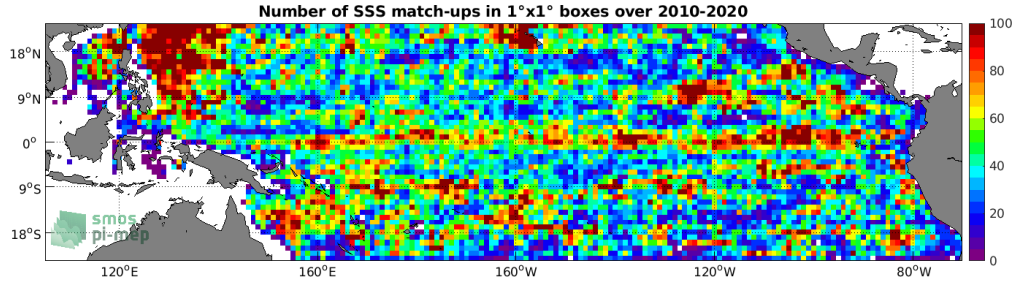
Figure 4: Number of SSS match-ups between Argo SSS and the SMOS SSS L3 v5 - 9 Days (CATDS-CECOS-LOCEAN) SSS product for the Tropical Pacific Ocean Pi-MEP region over 1^\circ \times 1^\circ boxes and for the full satellite product period.
