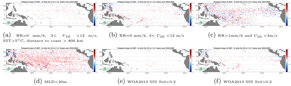
Figure 12: Temporal mean gridded over spatial boxes of size 1^\circ \times 1^\circ of \Delta SSS (SMOS SSS L3 v5 - 9 Days (CATDS-CECOS-LOCEAN) - Argo) for 6 different subdatasets corresponding to: RR=0 mm/h, 3 < U_{10} < 12 m/s, SST > 5^\circ C , distance to coast > 800 km (a), RR=0 mm/h, 3 < U_{10} < 12 m/s (b), RR > 1 mm/h and U_{10} < 4 m/s (c), MLD < 20 m (d), WOA2013 SSS Std < 0.2 (e), WOA2013 SSS Std > 0.2 (f).
