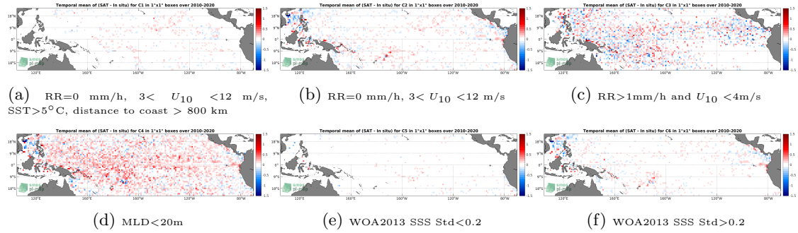
Figure 12: Temporal mean gridded over spatial boxes of size 1^\circ \times 1^\circ of \Delta SSS (SMOS SSS L3 v5 - 9 Days (CATDS-CECOS-LOCEAN) - Argo) for 6 different subdatasets corresponding to:RR=0 mm/h, 3 < U_{10} < 12 m/s, SST >5^\circ C, distance to coast > 800 km (a), RR=0 mm/h, 3 < U_{10} < 12 m/s (b), RR >1 mm/h and U_{10} < 4 m/s (c),MLD <20 m (d),WOA2013 SSS Std <0.2 (e),WOA2013 SSS Std >0.2 (f).
