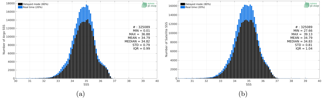
Figure 2: Histograms of SSS from Argo (a) and SMOS SSS L3 v5 - 9 Days (CATDS-CECOS-LOCEAN) (b) considering all match-up pairs per bins of 0.1 over the Tropical Pacific Ocean Pi-MEP region and for the full satellite product period.
